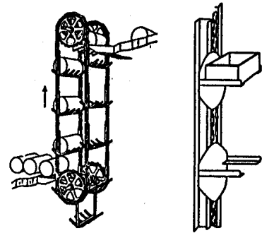
Fig. 10 — Suspended Tray Conveyors
