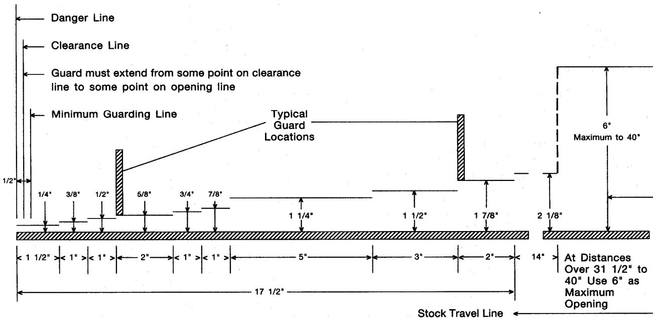
FIGURE 4 POSITIONING OF GUARD
