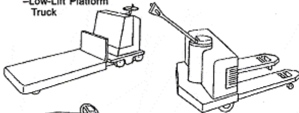
Fig. 4 -Motorized Hand Truck -Pallet Truck
