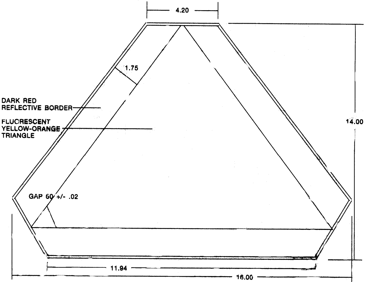
SLOW MOVING VEHICLE IDENTIFICATION SIGN
