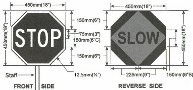
Detail of Paddle Sign
