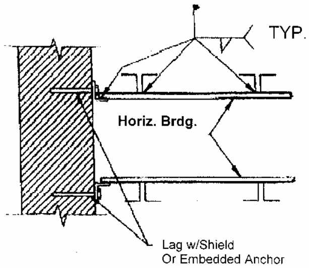
Horizontal Bridging Terminus at Wall
