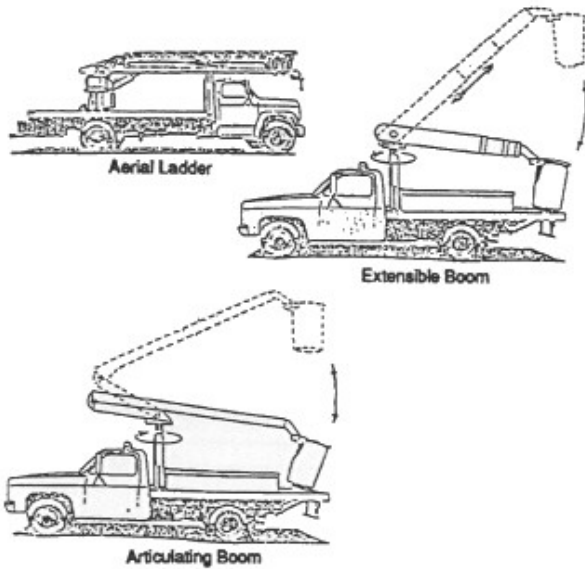
FIGURE 3 BOOM-SUPPORTED ELEVATING WORK PLATFORMS
