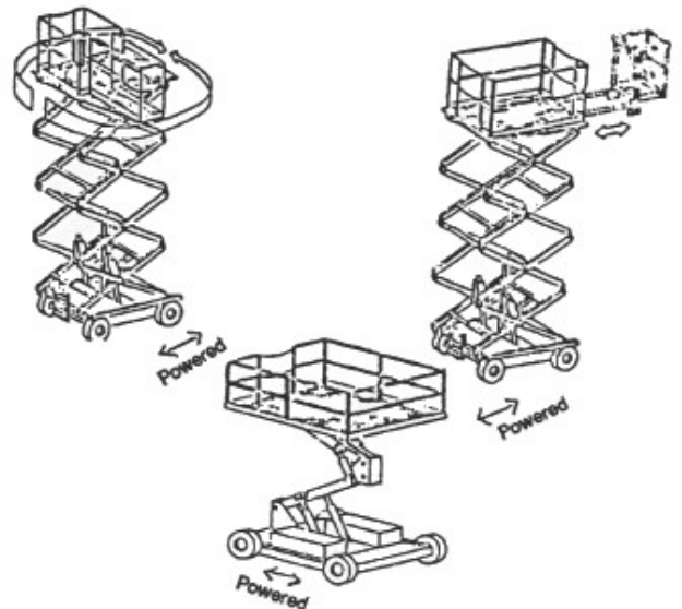
FIGURE 4 SELF-PROPELLED ELEVATING WORK PLATFORMS
