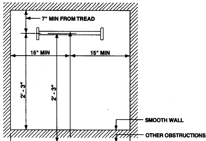
FIGURE 7 CLEARANCE DIAGRAM FOR FIXED LADDER IN WELL
