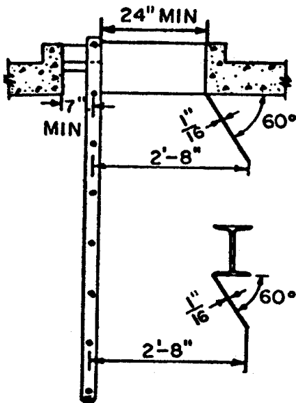
Figure 4 Deflector Plates For Head Hazards
