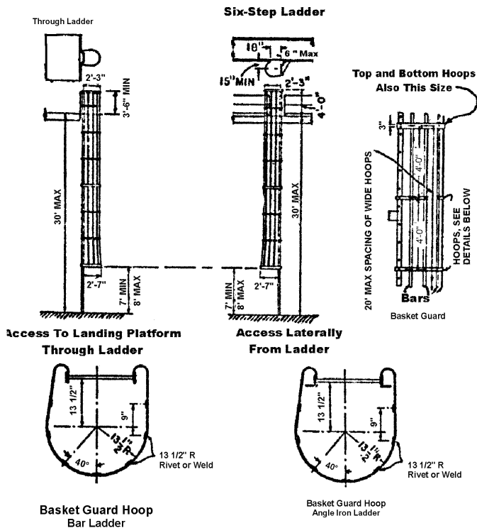
Figure 6 Cages for Ladders More Than 20 ft. High
