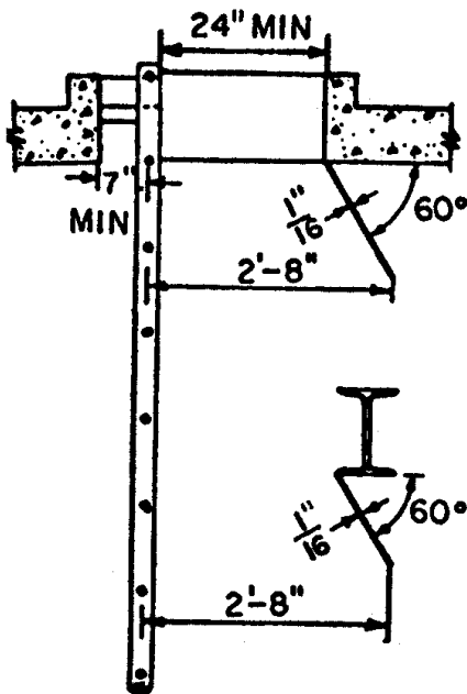
Figure 4 Deflector Plates For Head Hazards
