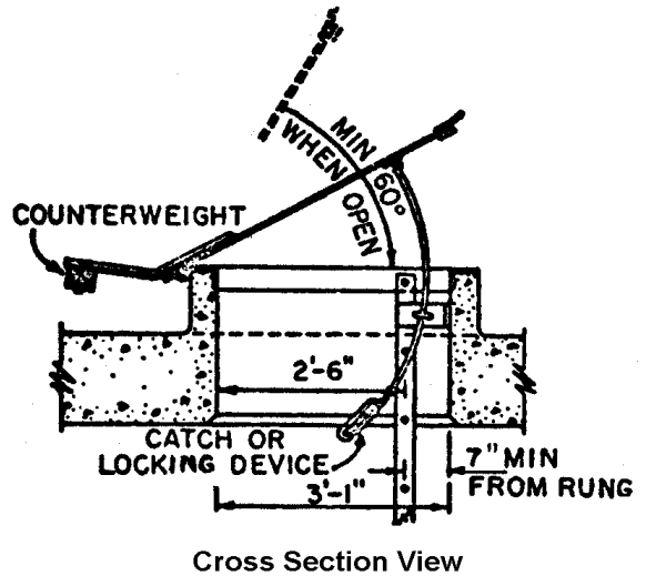
Figure 5 Relationship of Fixed Ladder to a Safe Access Hatch
