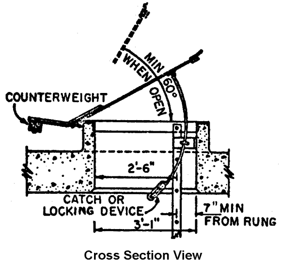
Figure 5 Relationship of Fixed Ladder to a Safe Access Hatch
