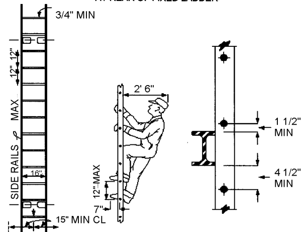
RAIL LADDER WITH BAR STEEL RAILS AND ROUND STEEL RUNGS
