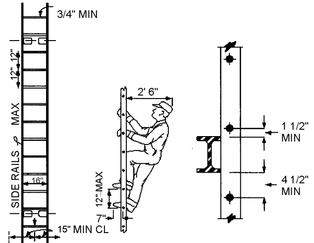
RAIL LADDER WITH BAR STEEL RAILS AND ROUND STEEL RUNGS
