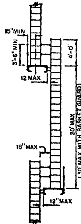
FIGURE 8 OFFSET FIXED LADDER SECTIONS
