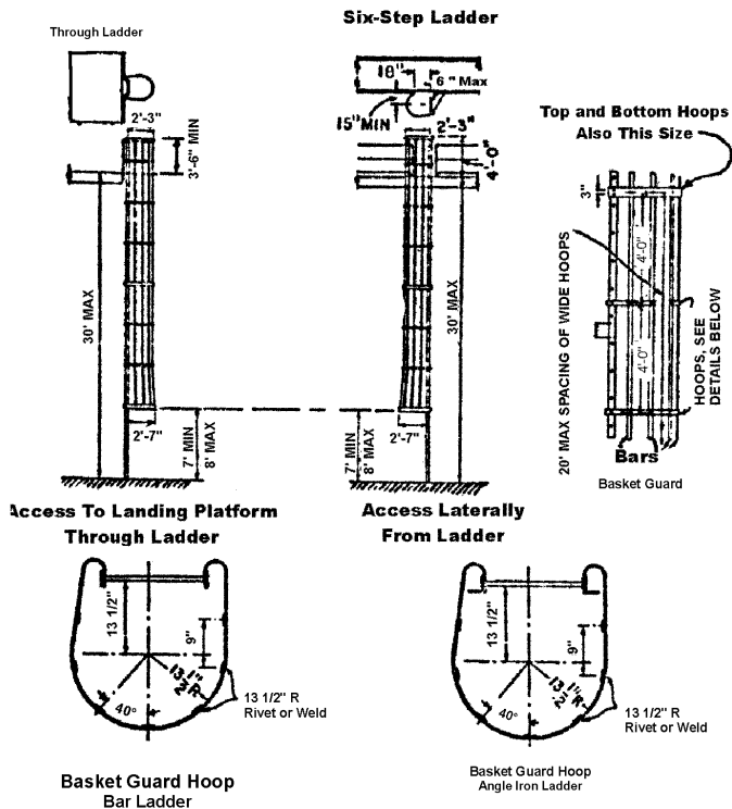
Figure 6 Cages for Ladders More Than 20 ft. High
