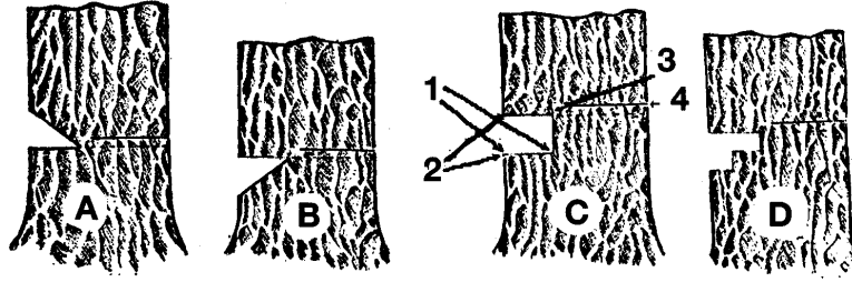
Figure 1 APPROVED UNDERCUTS
