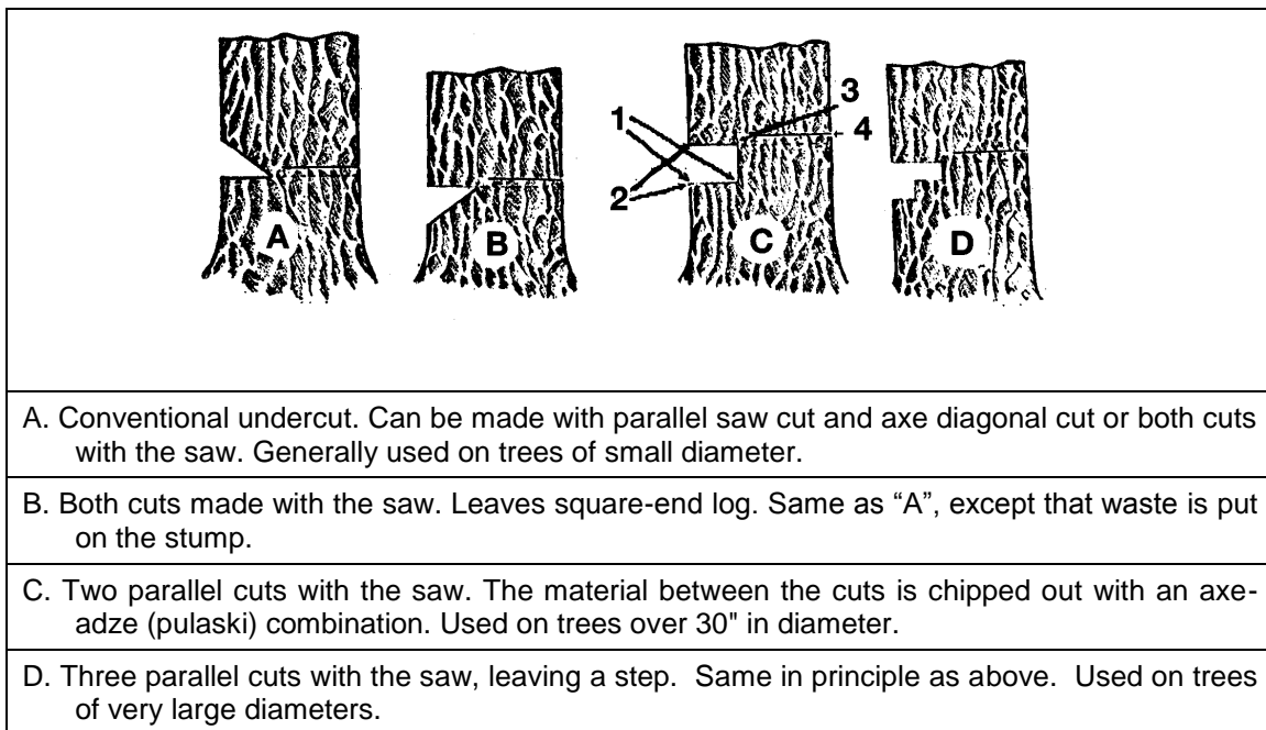
FIGURE 1 APPROVED UNDERCUTS
