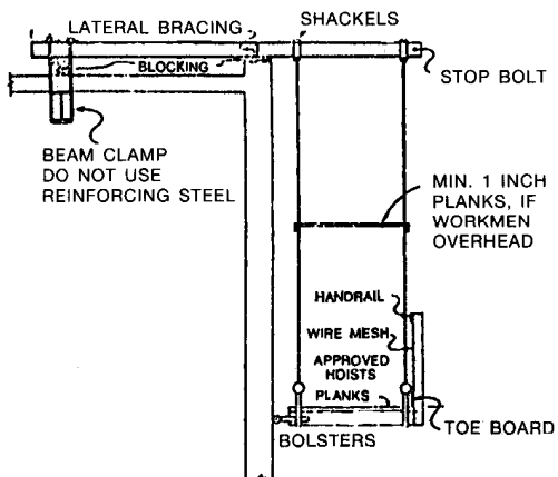
Suspension Scaffold Example 19
