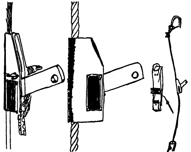
Fall Prevention Device Example 5
