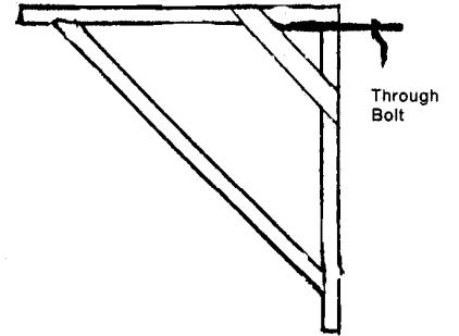
Carpenter's Bracket Scaffold Example 3
