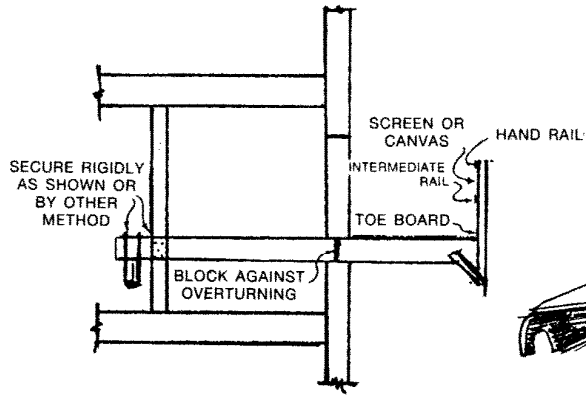
Outrigger Scaffold Example 13
