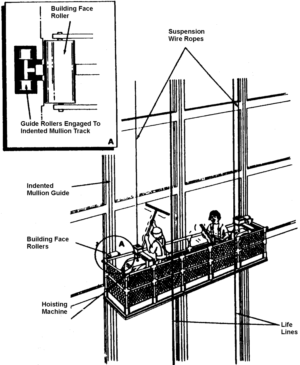
Typical Self-Powered Platform-Continuous External or Indented Mullion Guide System Example 23
