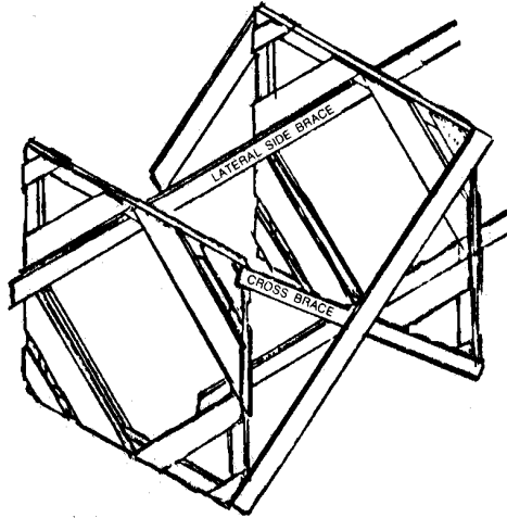
Bricklayer's Square Scaffold Example 2
