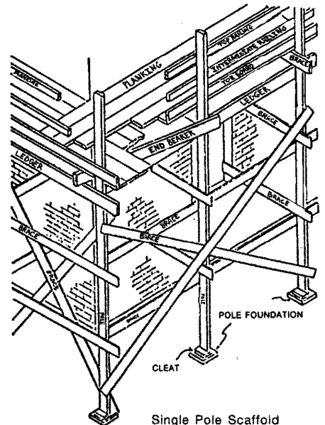
Single Pole Scaffold Example 18
