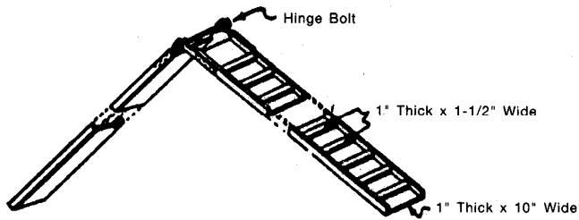
Crawling Board Example 4
