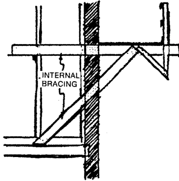
Outrigger Scaffold Example 13
