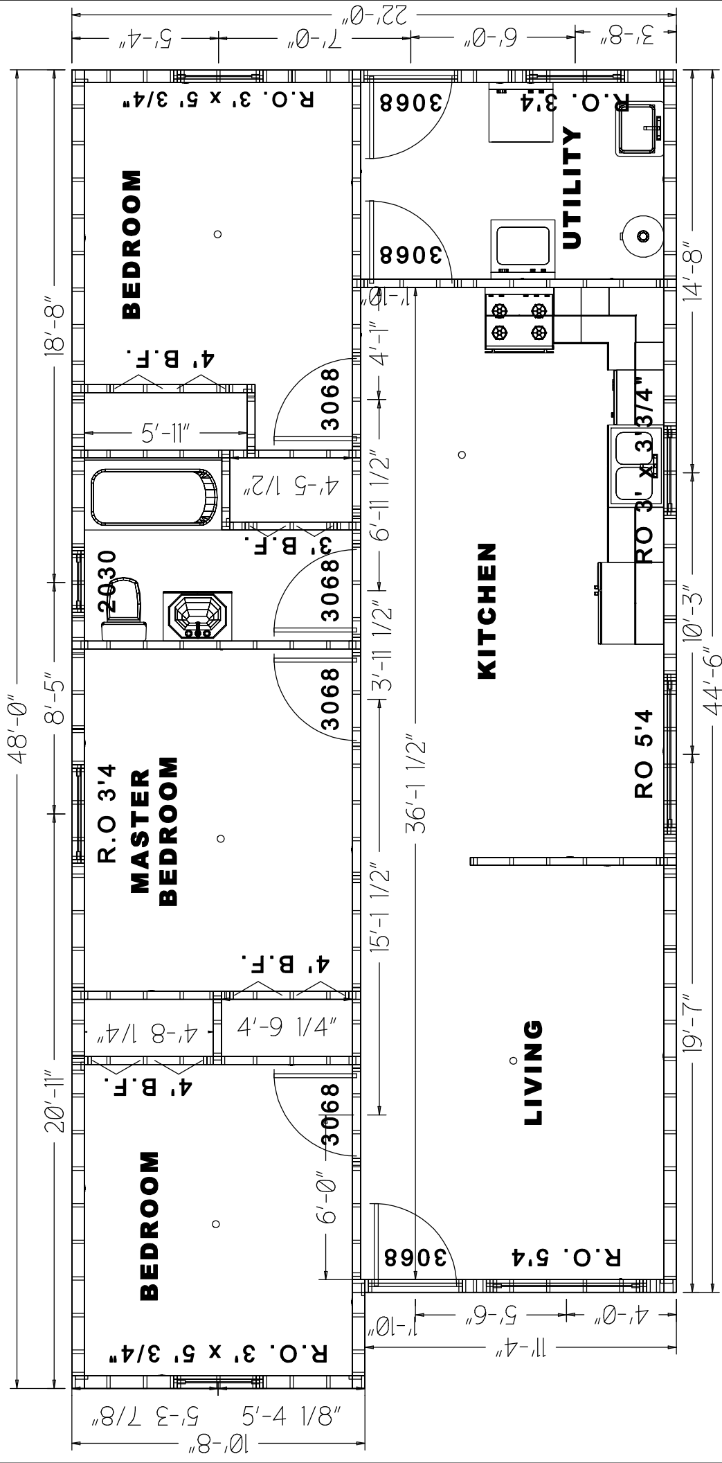
Carmack Shotgun House 2x6 16"O.C. Door & Window Openings & Dimensions
