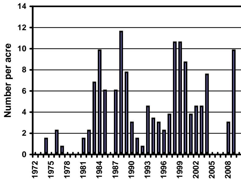
BROOK TROUT : Fall number/acre of fish from 8.0 - 11.9 inches long at Smith Bridge South Branch Au Sable River 1974 - 2009
