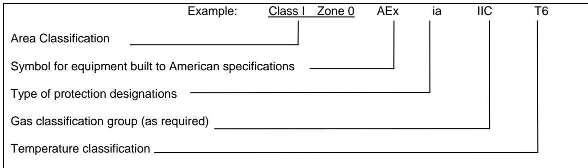
Figure S-1—Example Marking for Class I, Zone 0, AEx ia IIC T6
