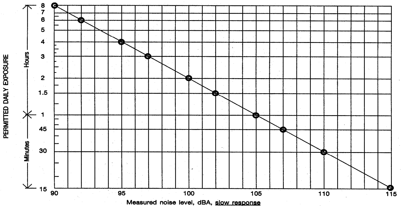
Chart A NOISE EXPOSURE CHART
