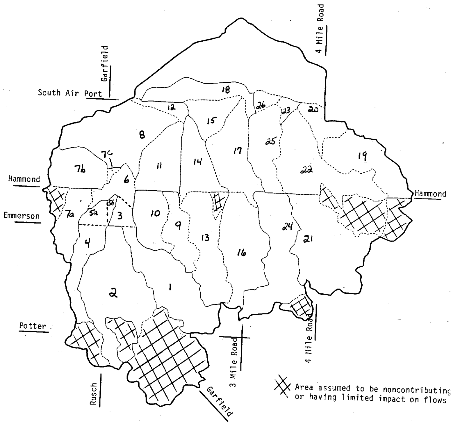
FIGURE 3 SUBWATERSHED BOUNDARIES
