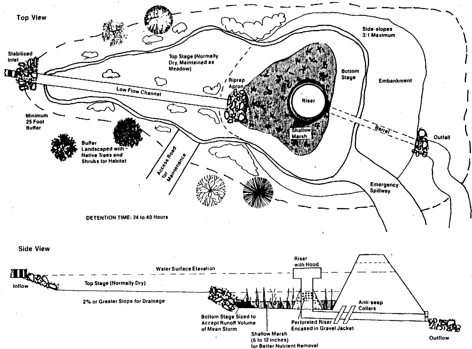
Figure 8 - Extended Detention Pond
