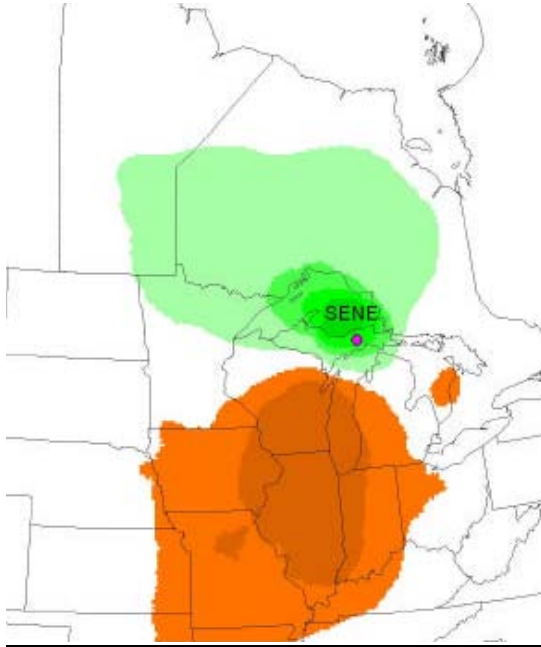
Figure 10.2.c: Composite back trajectories for Seney for the 20% worst days. Orange is where the air is most likely to come from and green is where it is least likely to come from.
