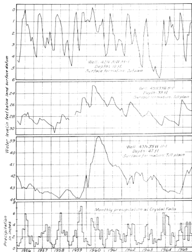
Figure 3. Fluctuations of ground-water levels.
