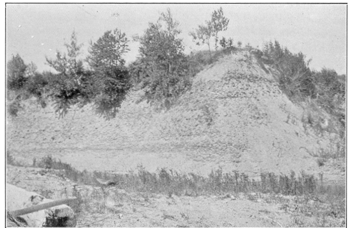
Plate III. (b) Shale near White Rock, about 2½ miles north of Forestville.
