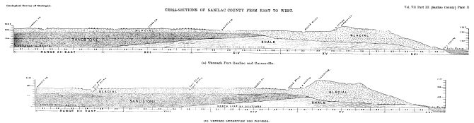
Plate II. Cross-sections of Sanilac county from east to west. (a) Through Port Sanilac and Carsonville. (b) Through Deckerville and Novesta.
