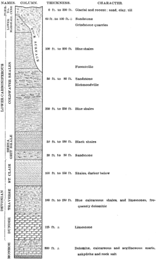
Figure 1. General section of rock formations underlying Sanilac county.
