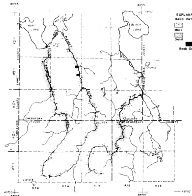
Figure 14. Low banks are chiefly muck; higher banks are predominately sand.
