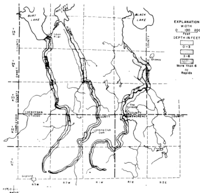
Figure 10. Stream widths vary, but generally increase in the downstream direction. Upper reaches of streams in study area are shallow; shoals and deeps alternate in lower reaches.
