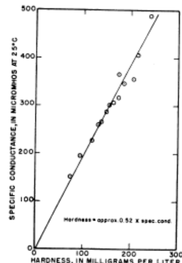
Figure 57. Hardness of river water in the study area, in milligrams per liter, is about half the value of specific conductance, in micromhos at 25°C.
