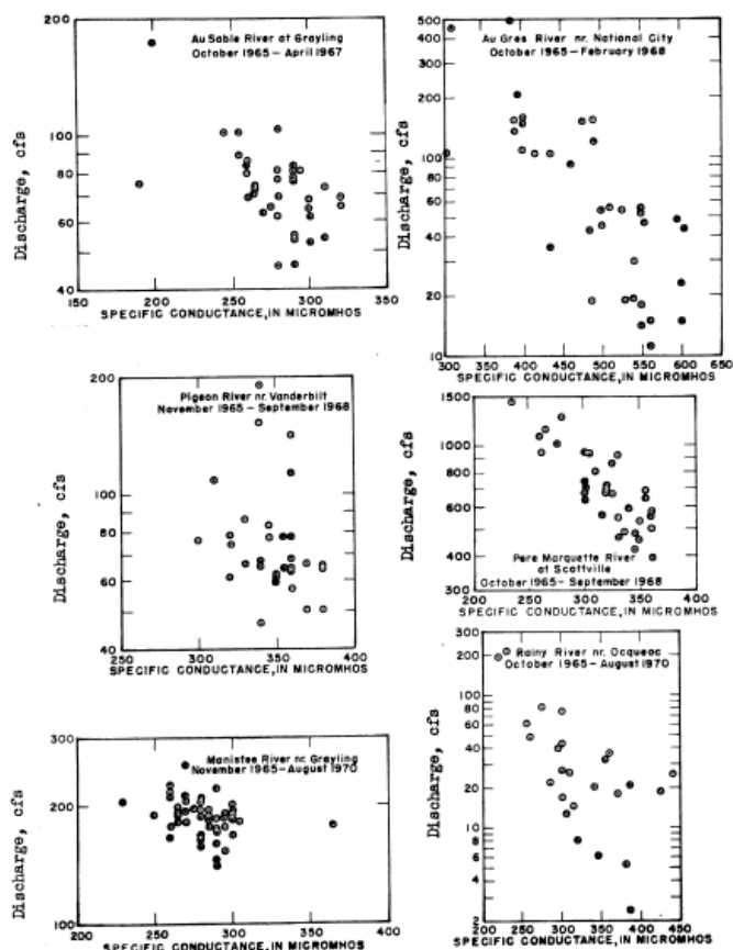
Figure 59. Specific conductance usually declines with increased discharge on streams, such as Au Gres, having substantial amounts of surface runoff. This relationship is not well-defined on streams with very little surface runoff, such as the Manistee.
