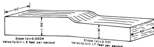
Figure 17. When the gradient of a river increases, velocity of streamflow usually increases and cross-sectional area decreases.
