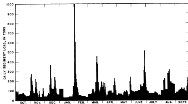
Figure 55. Sediment load (suspended sediment and bed load) of the Pine River near Wellston varied from 30 to 997 tons per day (October, 1967 to September, 1968).
