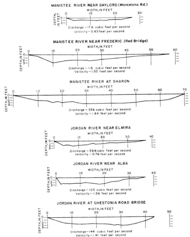
Figure 9. Cross-sectional areas of streams generally increase downstream with increasing discharge.
