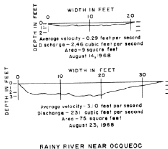
Figure 12. The cross-sectional area of the Rainy River increased about 8 times when surface runoff from heavy rains reached the stream.
