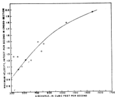
Figure 29. Velocity of flow increases when discharge increases.
