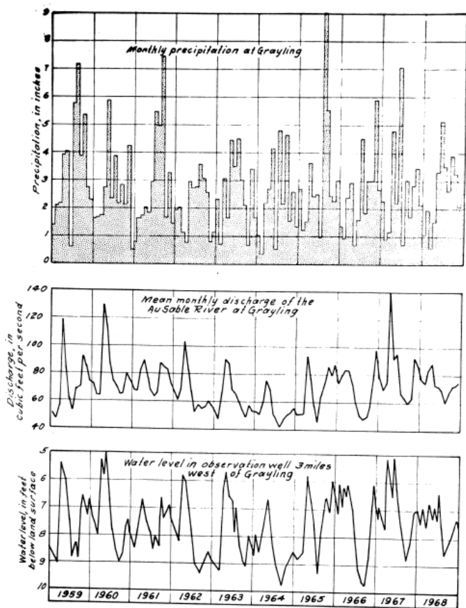
Figure 3. Ground-water levels rise and streamflow increases in response to spring snowmelt and heavy rains. The influence of rainfall is relatively small during the growing season.
