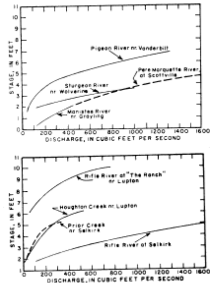
Figure 28. Increasing discharge is marked by rising stage.
