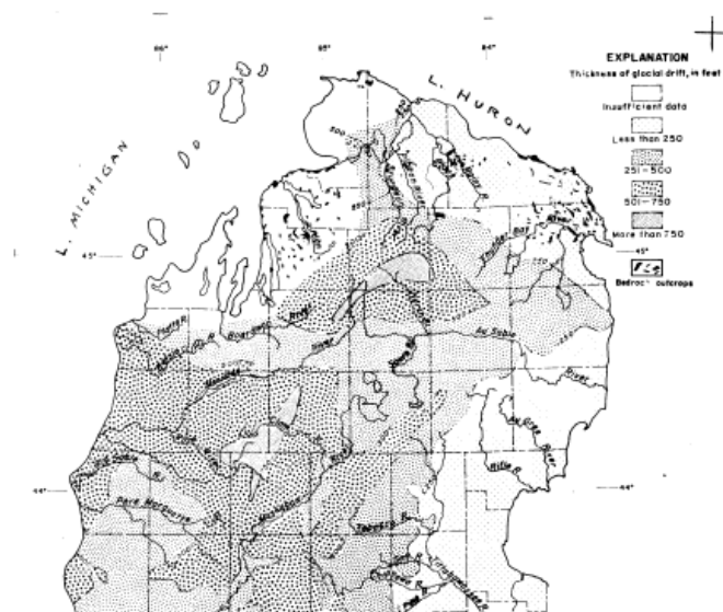
Figure 7. Glacial drift is several hundred feet thick in most of study area, but is thin or absent in places near the Great Lakes shorelines.
