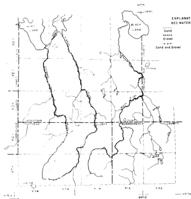
Figure 20. Sand and gravel beds alternate in varying proportions.
