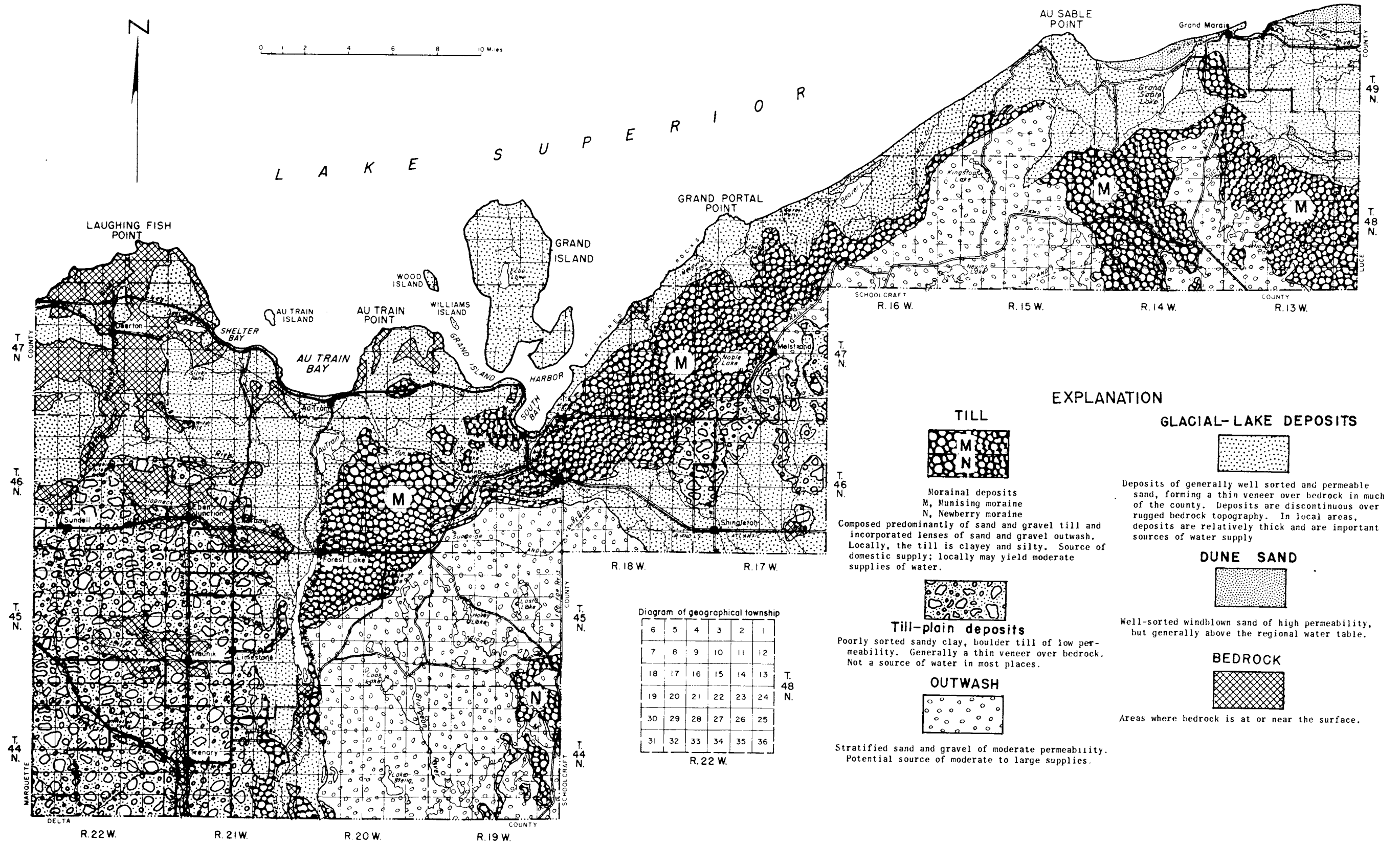
Figure 8.--Surface geology of Alger County (adapted from Bergquist, 1936, fig. 14).
