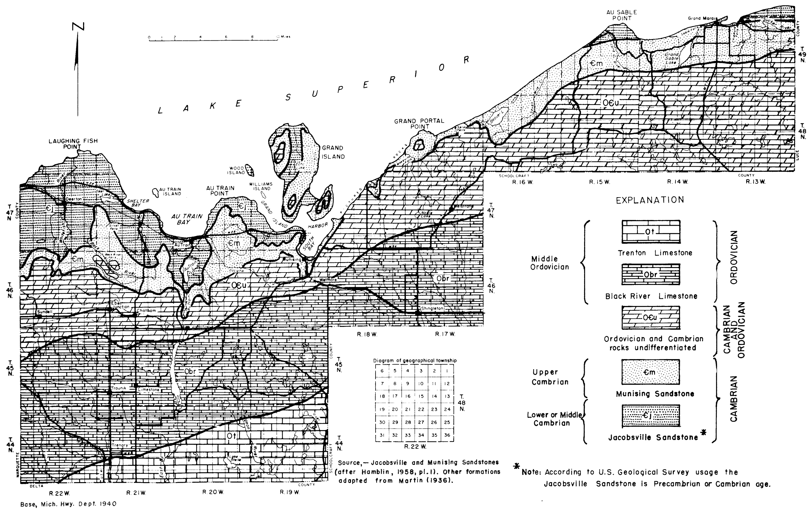
Figure 5.--Bedrock geology of Alger County.
