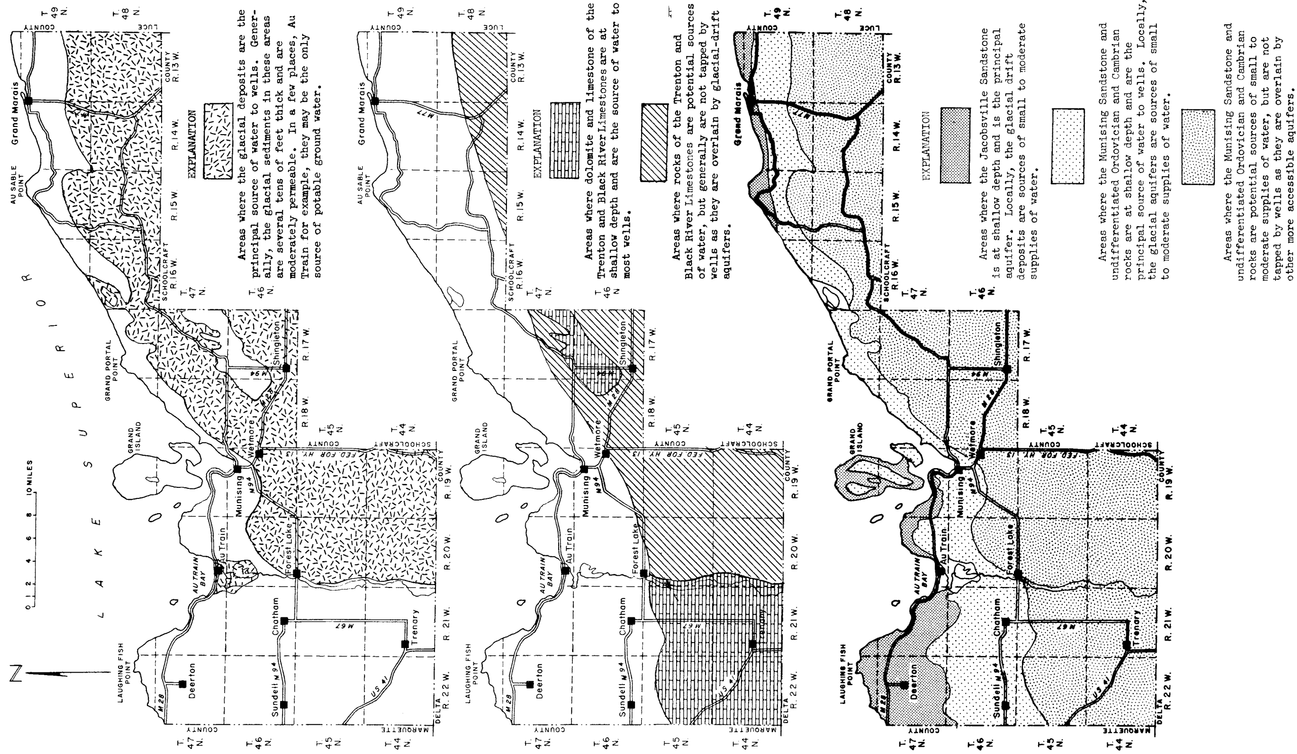
Figure 10.--Source and availability of ground water in Alger County.
