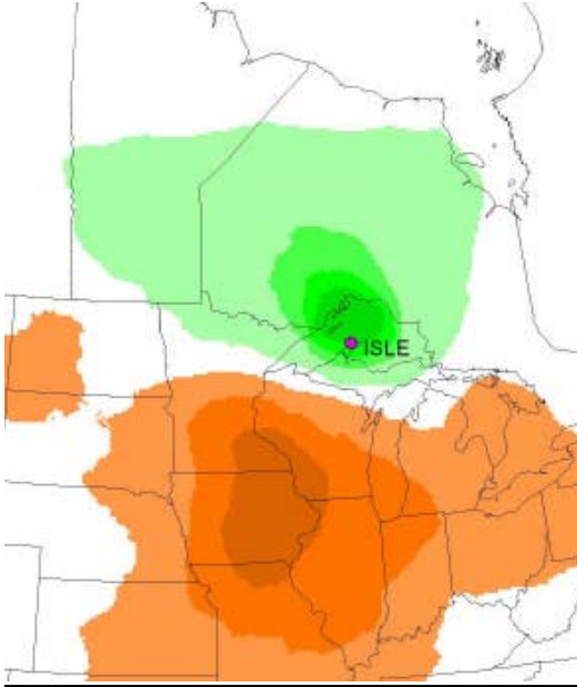
Figure 10.2.b: Composite back trajectories for Isle Royale for the 20% worst days. Orange is where the air is most likely to come from and green is where it is least likely to come from.
