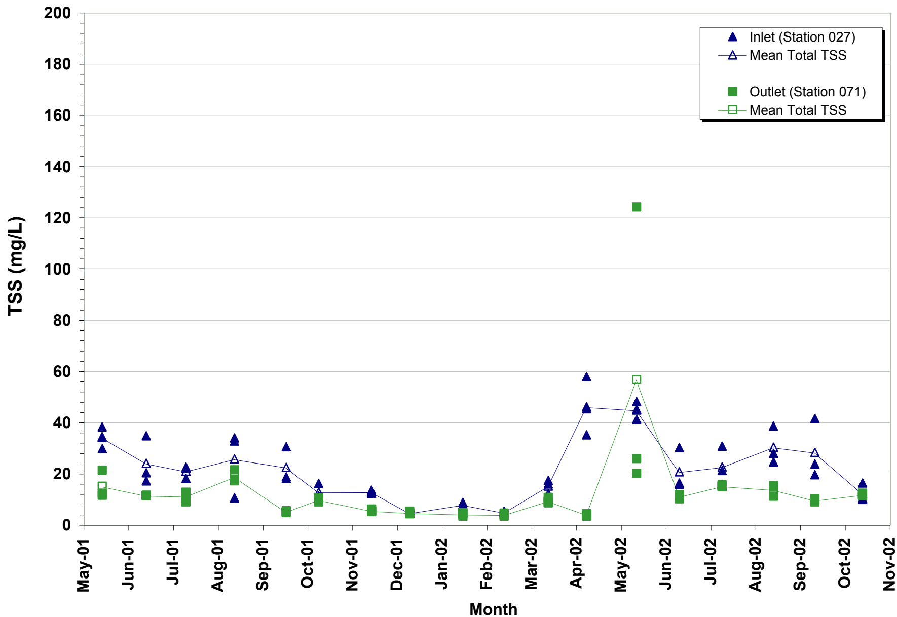
Figure 3-4. Total and Mean Total TSS Concentrations Lake Allegan Inlet - Outlet Stations May 2001 through October 2002
