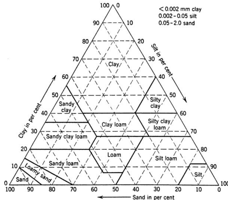
Figure 1-5 Textural Triangle
