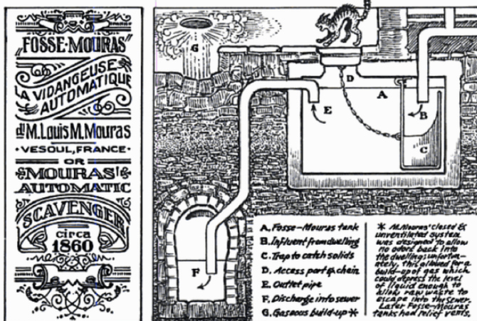
Fig 1. Schematic of an early-design septic tank from 1860. (from http://djwl.co.uk/blog/brief-history-septic-tanks/ )
