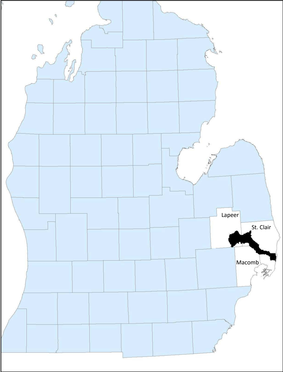
Figure 1.-Location map for the Belle River watershed.
