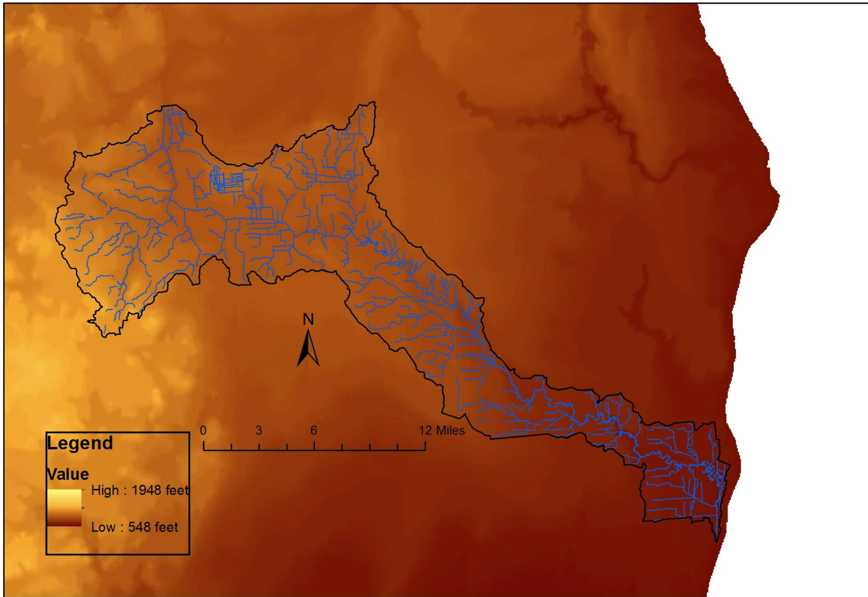
Figure 4.-Digital Elevation Model of the Belle River watershed.
