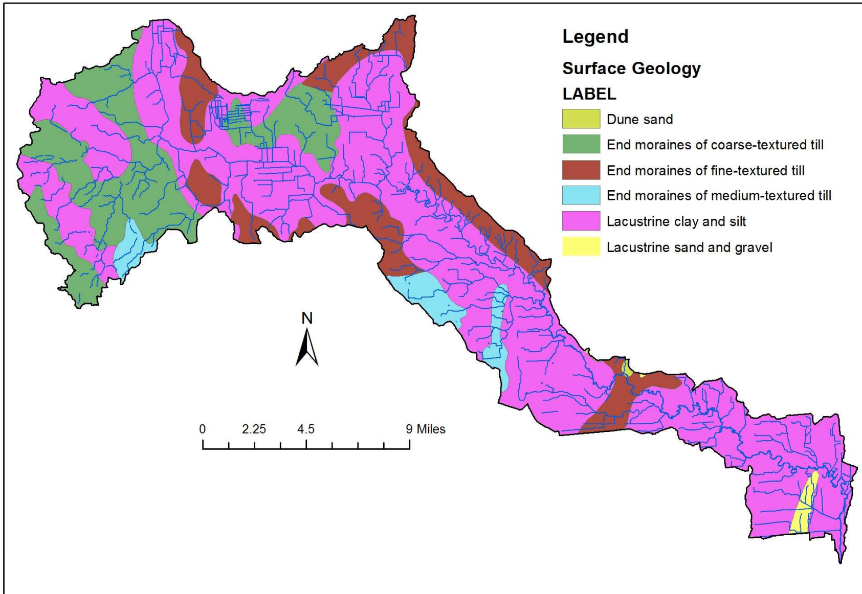
Figure 3-Surface geology map of the Belle River watershed.
