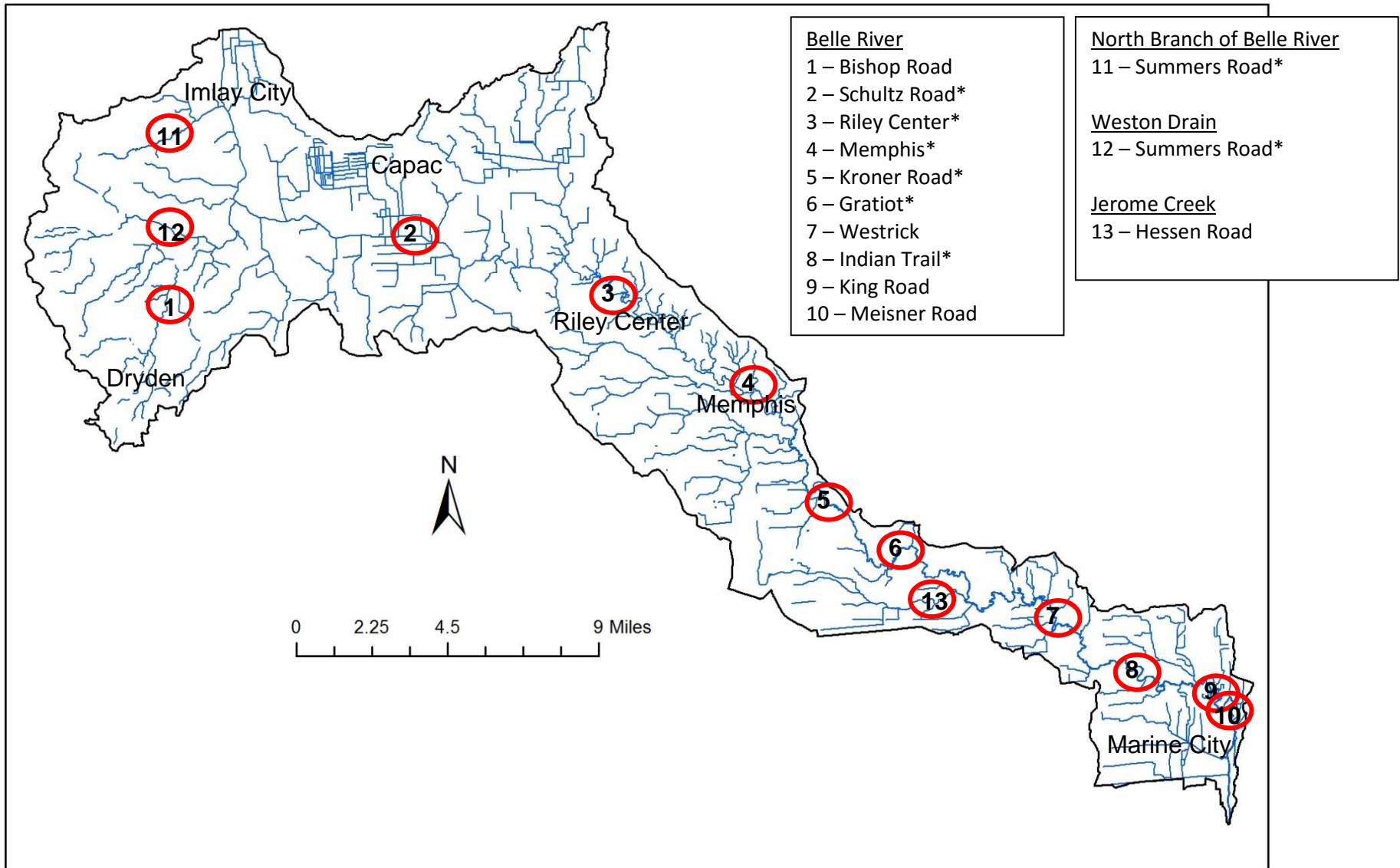
Figure 2.-Map of the Belle River watershed, with locations where fish surveys were conducted in 2008. Sites indicated with an asterisk also had temperature data collected in 2010.
