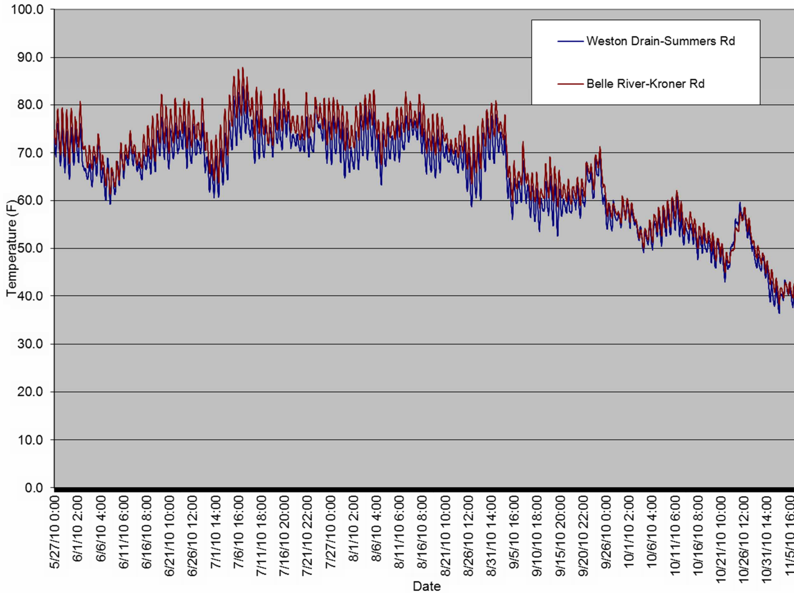
Figure 5. Water temperature from the Belle River.
