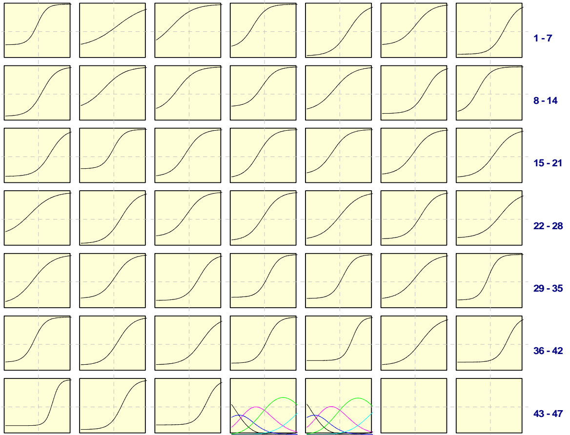
Matrix Plot of Item Characteristic Curves: MME S10 Writing Initial Form
