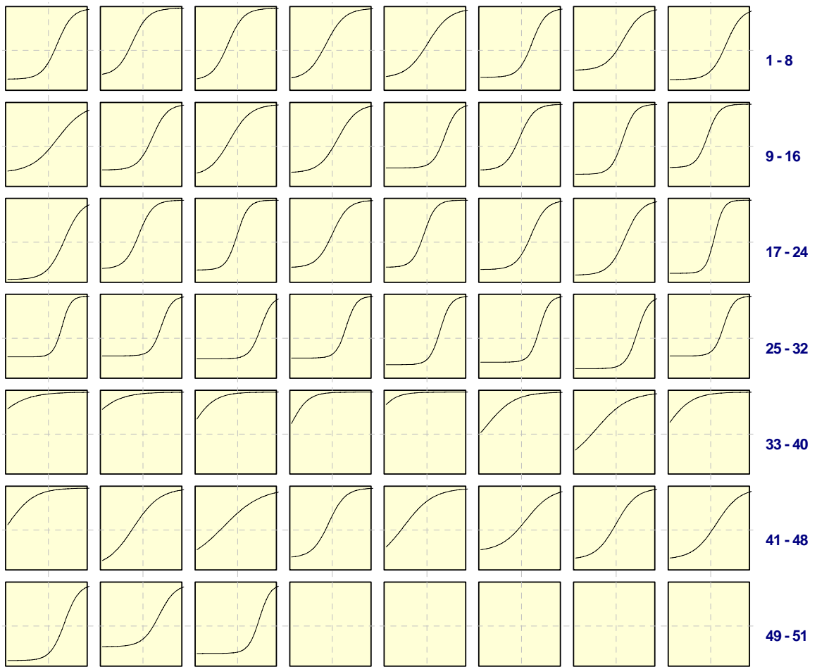
Matrix Plot of Item Characteristic Curves: MMES10 Reading Initial Form
