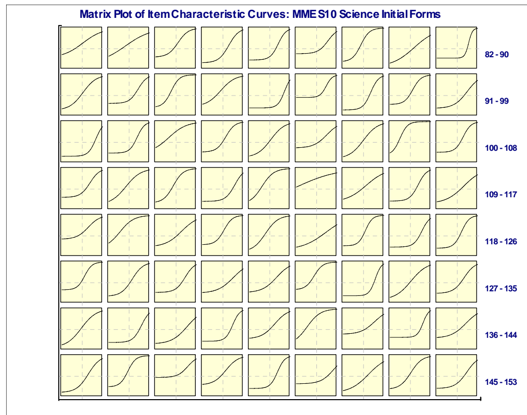
Figure 8.4. Item Characteristic Curves – Science Spring 2010: 20 selected ACT Science items plus 133 unique Michigan-developed Science items.
