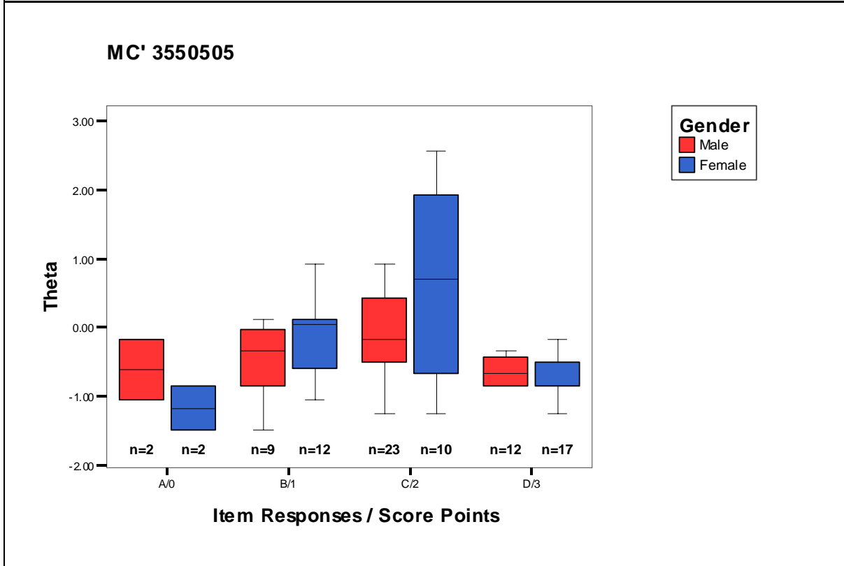
Figure 12.2a. Box & Whisker plots for ethnicity and gender for MC items.
