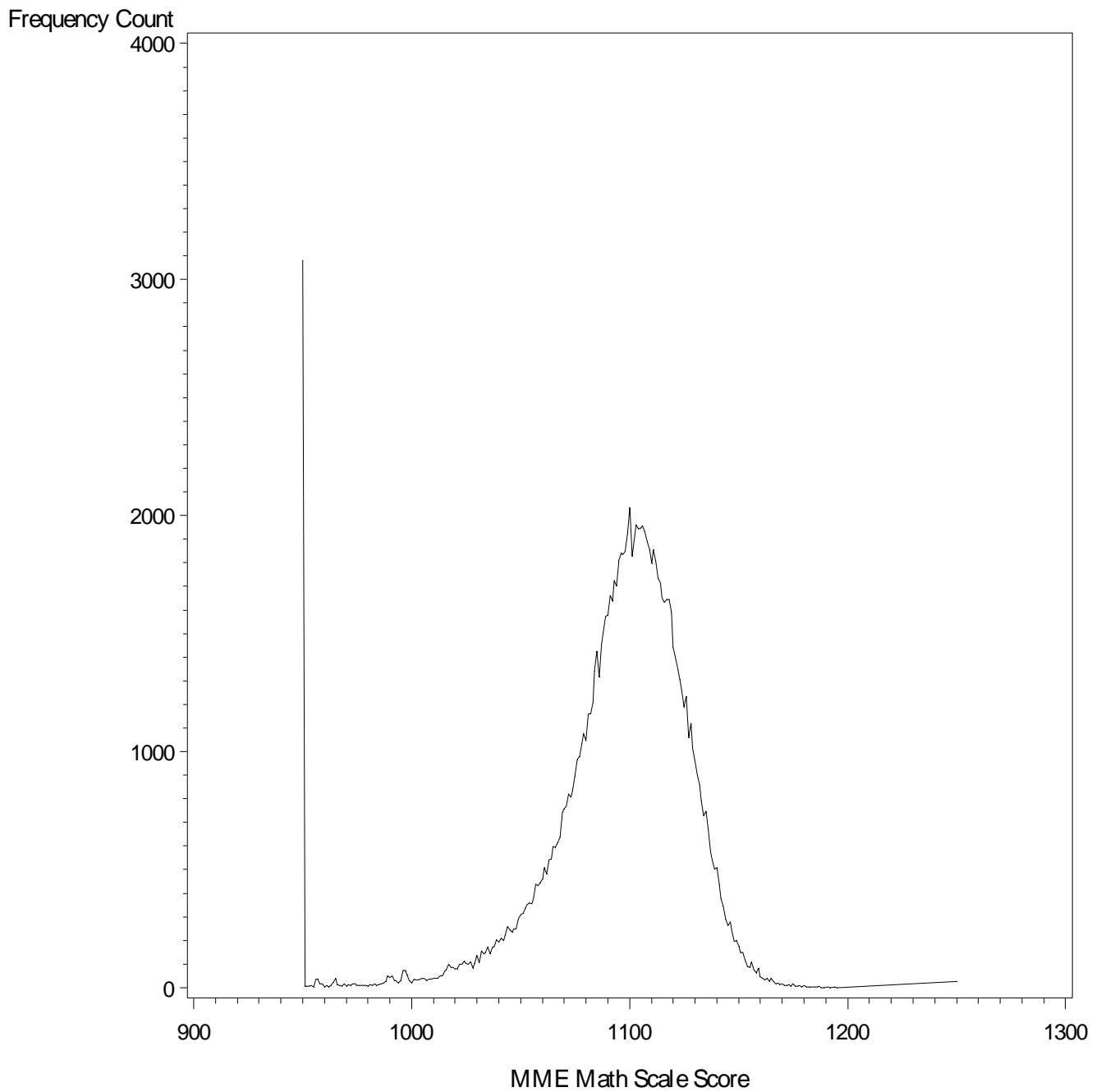
Figure 15.1. Frequency plot for MME Spring 2010 Mathematics scale score total group – All forms included.
