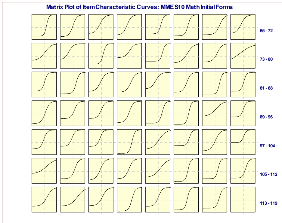
Figure 8.3. Item Characteristic Curves – Mathematics Spring 2010: 36 selected ACT Mathematics items plus 12 selected WorkKeys Applied Mathematics items plus 3 selected WorkKeys Locating Information items plus 68 unique Michigan-developed Mathematics items.
