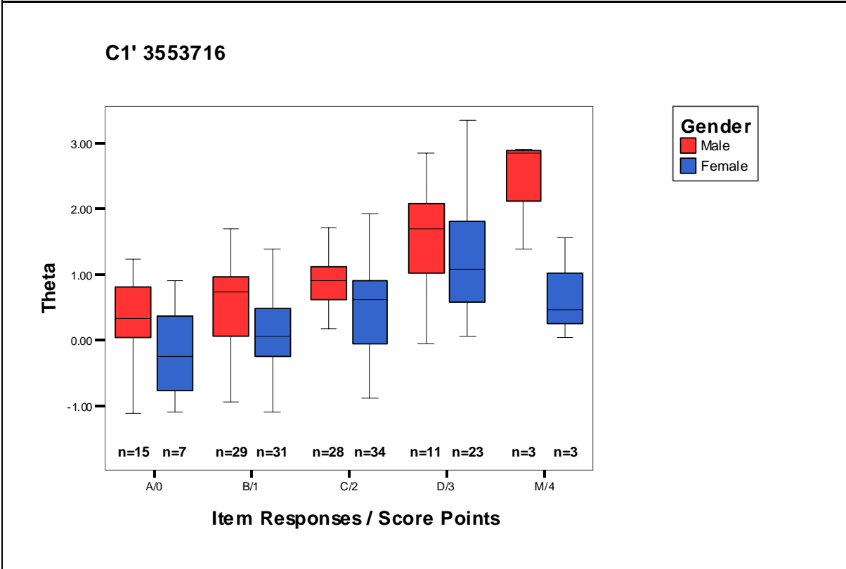
Figure 12.2b. Box & Whisker plots for ethnicity and gender for CR items.
