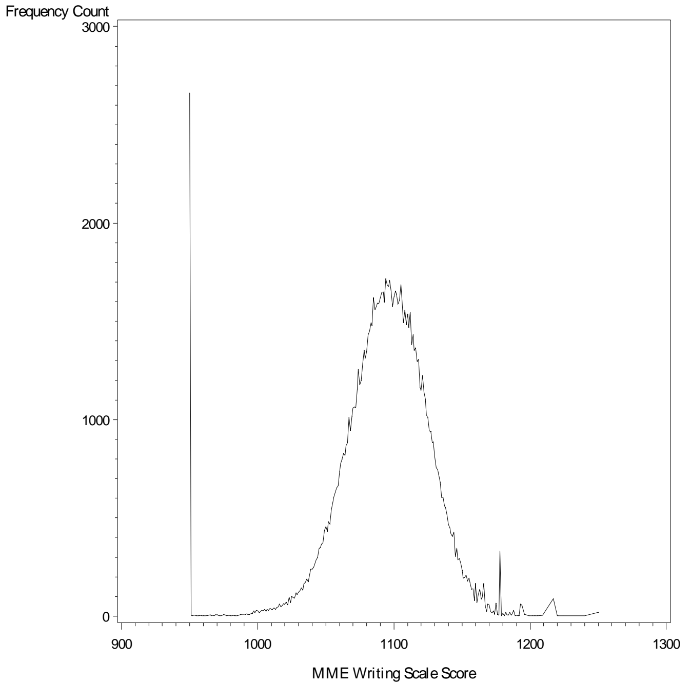
Figure 15.5. Frequency plot for MME Spring 2010 Writing scale score total group – All forms included.
