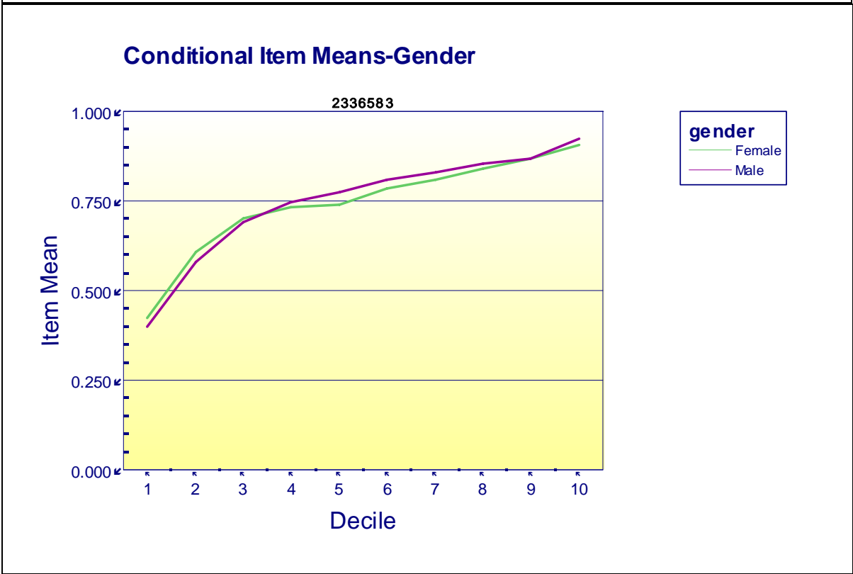
Figure 12.1a. Conditional item mean plots for ethnicity and gender for MC items.
