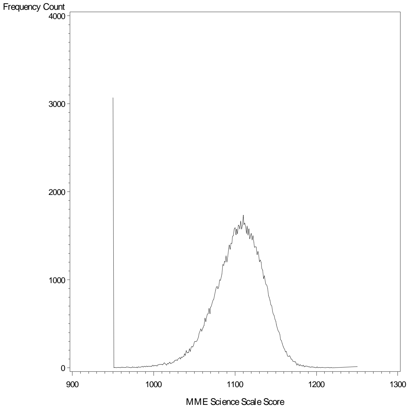
Figure 15.3. Frequency plot for MME Spring 2010 Science scale score total group – All forms included.
