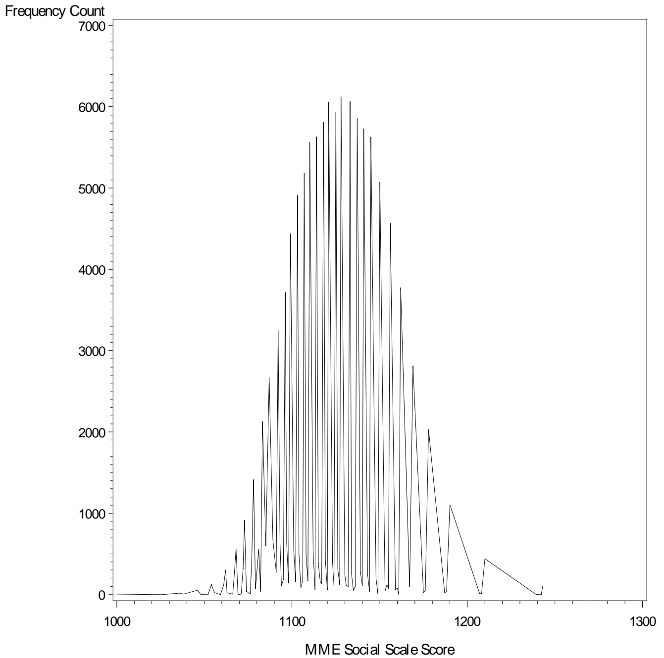
Figure 15.4. Frequency plot for MME Spring 2010 Social Studies scale score total group – All forms included.
