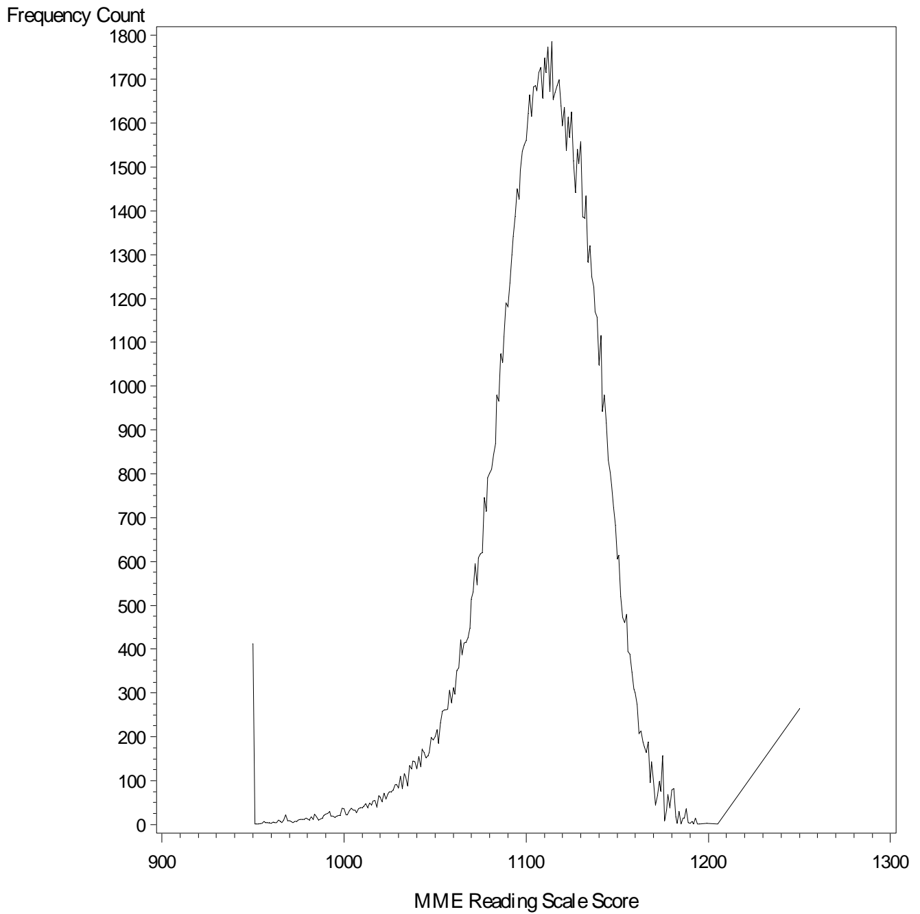
Figure 15.2. Frequency plot for MME Spring 2010 Reading scale score total group – All forms included.
