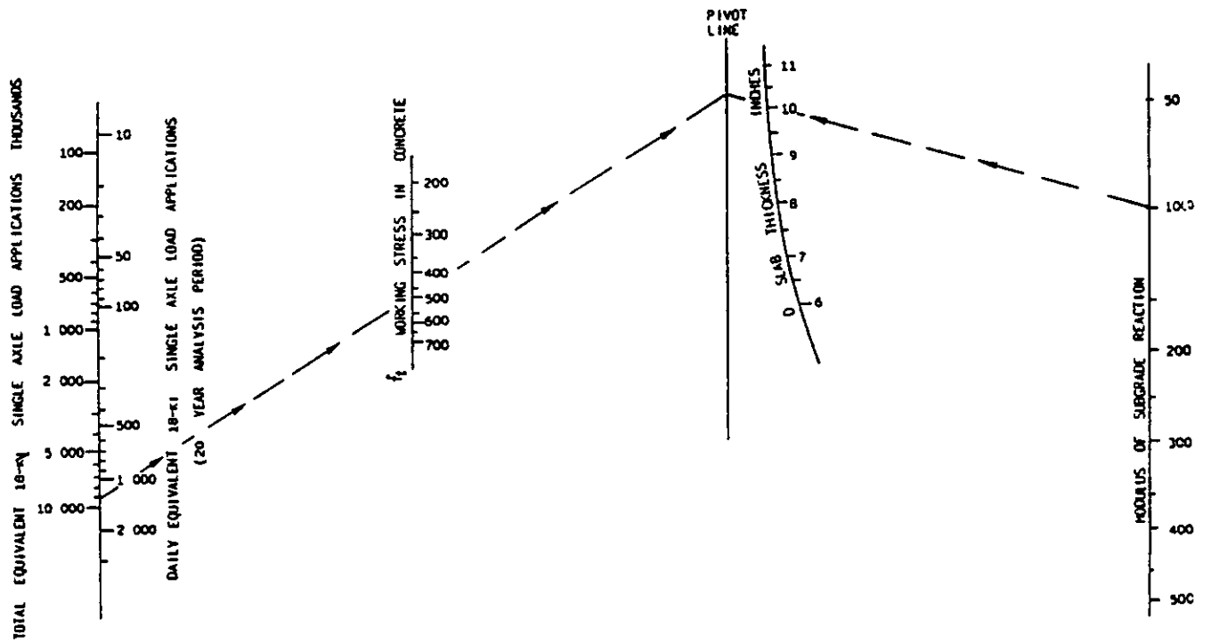
Figure III-1 Design Chart for Rigid Pavements p_t 2 5
