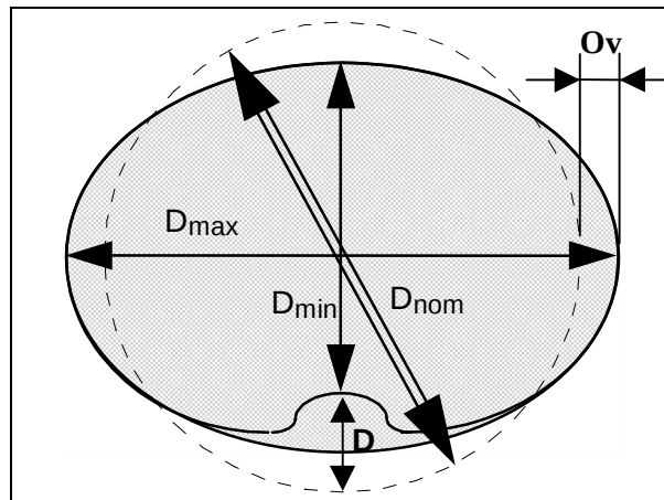
Figure 5.3 Anomaly Sizing
