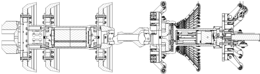
20" Mechanical Caliper GEOPIG™
