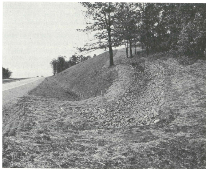
Figure 22: Cobblestone Ditch at Slope Interface
