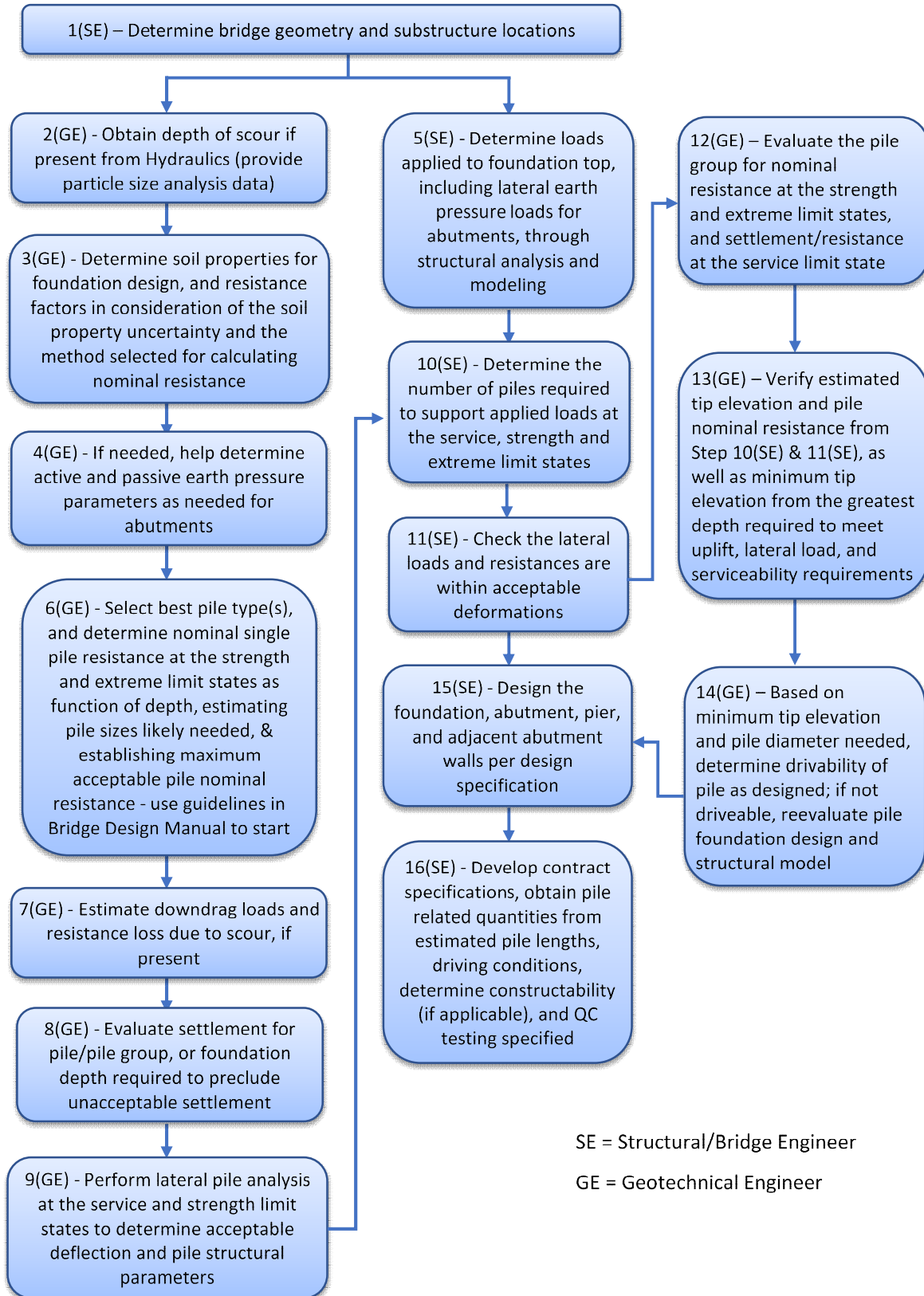
Figure 24: General Flowchart for LRFD Pile/Shaft Design
