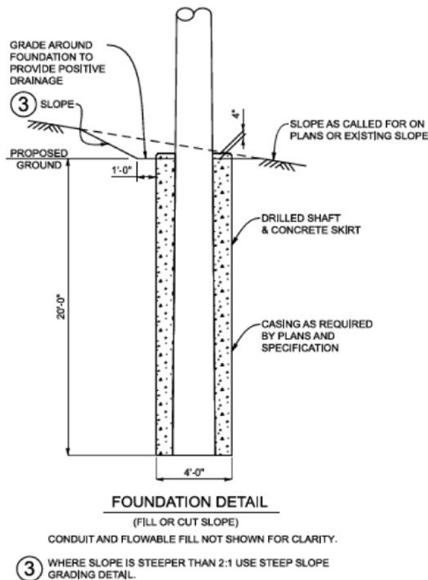
Figure 32: General Cross-Section of a CCTV Foundation
