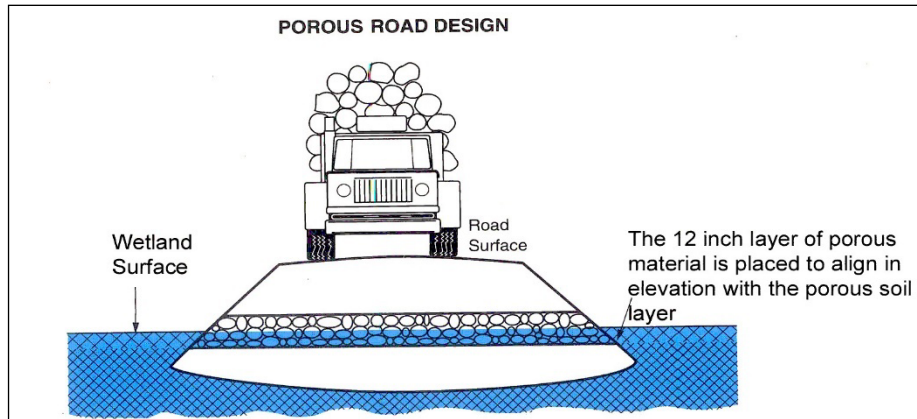
Figure 8. Porous Road Design Using Large Stone.
