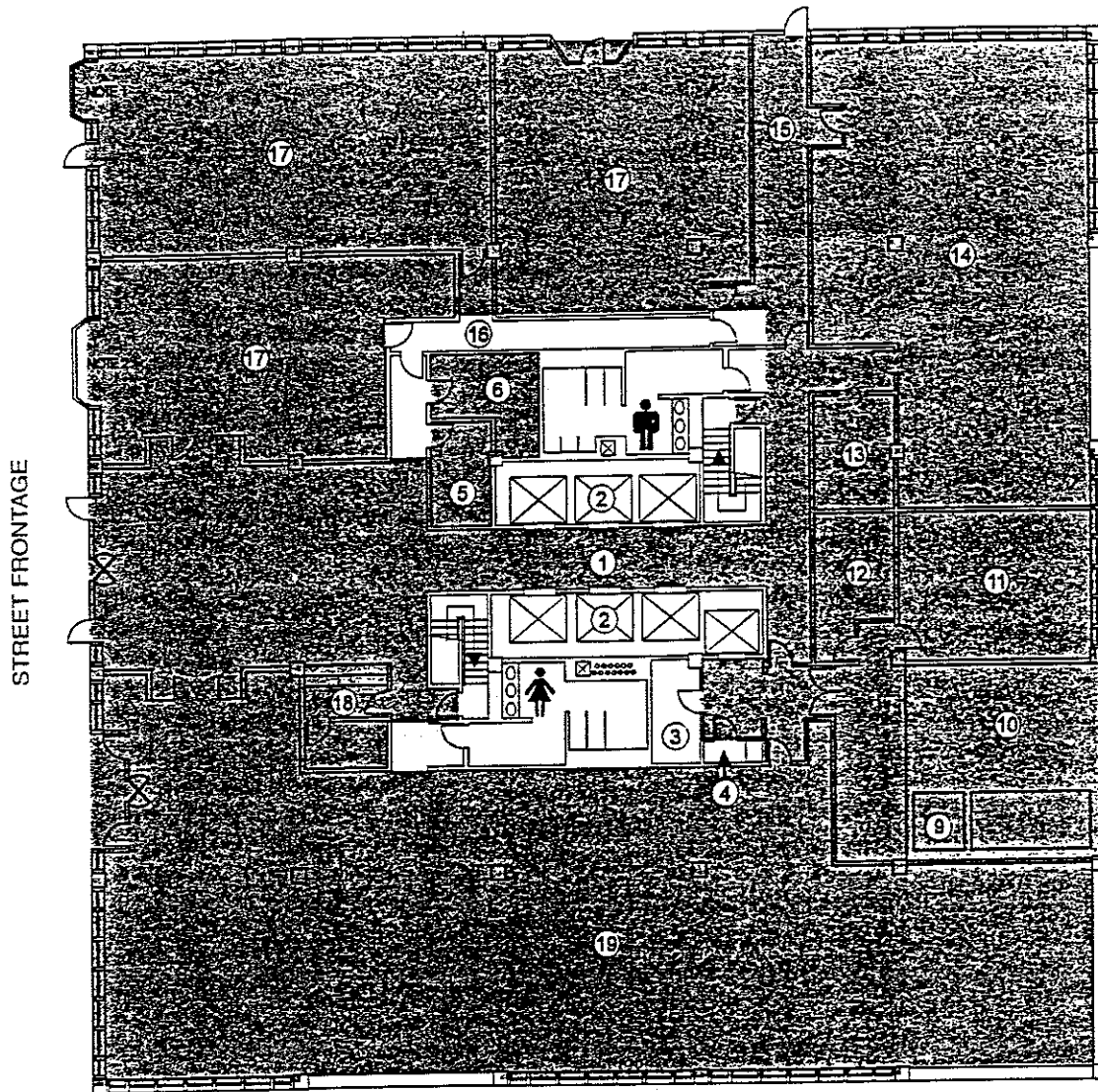
ILLUSTRATION OF FLOOR USABLE AREA FOR A TYPICAL GROUND FLOOR LEVEL WHERE THE BUILT AREA BOWS OUT OF AN OTHERWISE STRAIGHT BUILDING LINE (Note 1) AND A BAY WINDOW EXTENDS OUTSIDE THE BUILDING LINE (Note 2)
