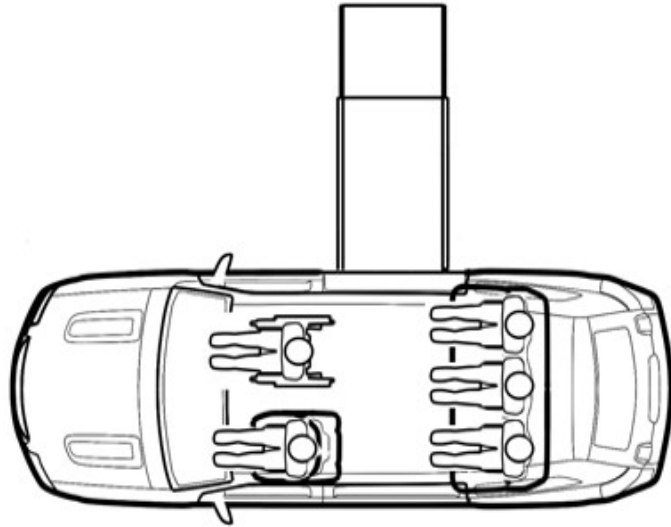
A. 3+2 Purpose Built Vehicle with ramp – vinyl (less single rear facing seat).
