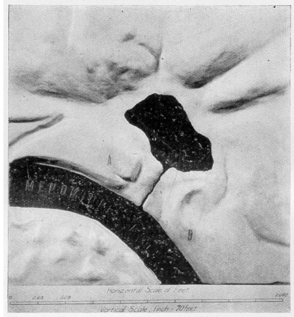
Plate XII. A. Model of gravel bars near Sturgeon Falls.
