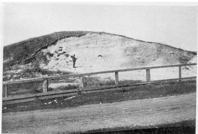
Plate XI. B. Section of an esker.
