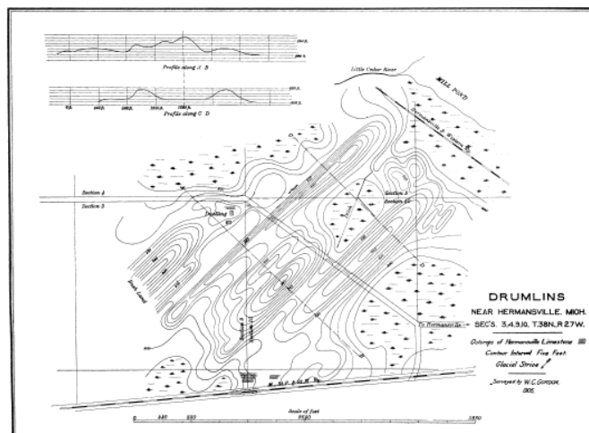
Plate VIII. Map of drumlins near Hermansville.
