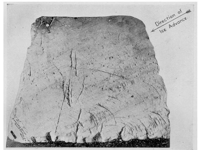
Plate IV. A. Crescentic cracks in quartzite.
