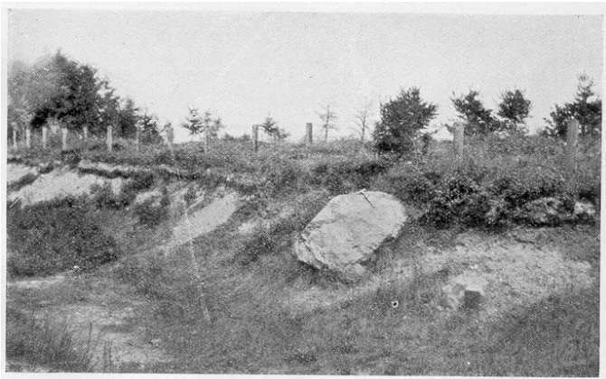
Plate VII. B. Boulders in a sand and gravel plain.
