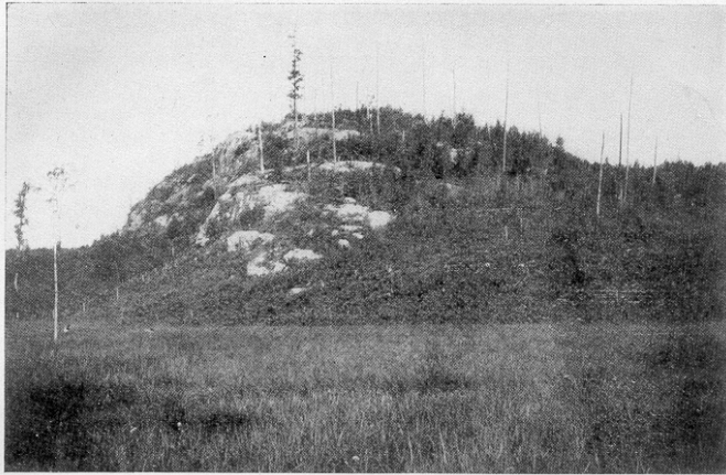
Plate VI. A. Glaciated hill showing stoss and lee sides.
