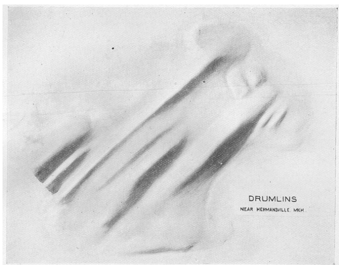
Plate IX. A. Model of drumlins near Hermansville.
