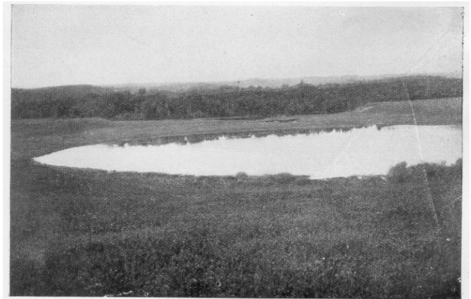
Plate XII. B. Gravel bars near Sturgeon Falls.
