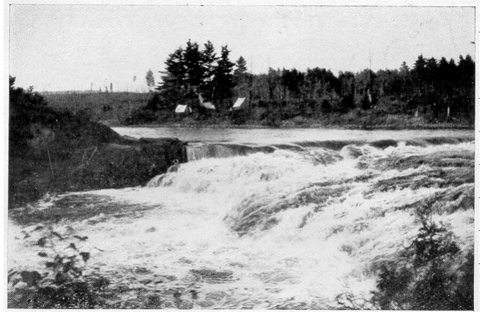
Plate I. A. Lower Twin Falls, Menominee River.
