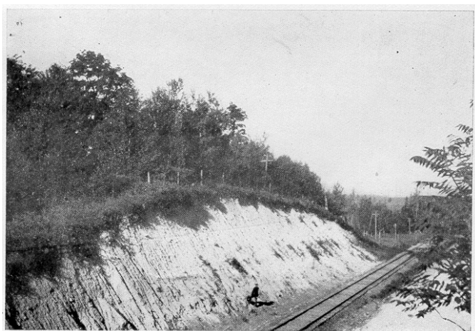
Plate IX. B. Section of drumlin.
