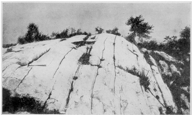
Plate V. A. Glaciated summit of quartzite ridge, viewed with the bedding.
