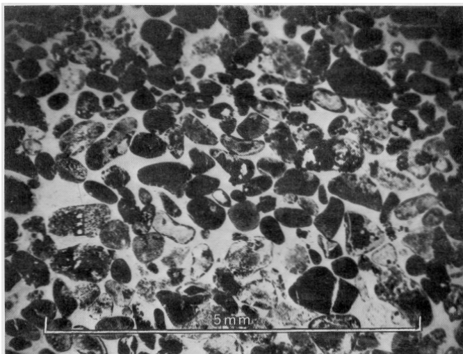
Figure 2.--Photomicrograph showing hematitic granular cherty iron-formation from Anvil Member, Ironwood Iron-formation; NW¼NW¼ sec. 13, T. 47 N., R. 46 W., near Ramsay, Mich.; plane-polarized light.
