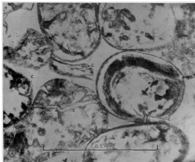
Figure 6.--Photomicrograph showing chert granules in the Anvil Member, Ironwood Iron-formation; plane-polarized light. Some granules contain chert-filled spaces (c) that may be contraction cracks. The dark material is hematite. Drill hole 540, 47 m (155 ft) from hole collar, Peterson mine, Yale, Mich.
