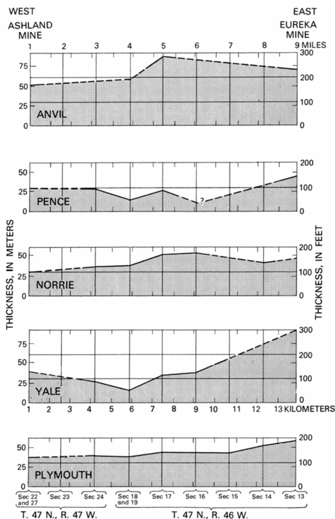
Figure 8.--Graphs showing thicknesses of the five members of the Ironwood Iron-formation between Ironwood and Ramsay, Mich. Thicknesses plotted on the vertical lines are averages of all data in a 1.6-km (1-mi) distance along strike. Thickness line is dashed where approximate. Numbers at the top are distances from the Michigan State line in miles and kilometers. (Thicknesses in the ninth column are average data from only 0.8 km (0.5 mi) of strike distance.)
