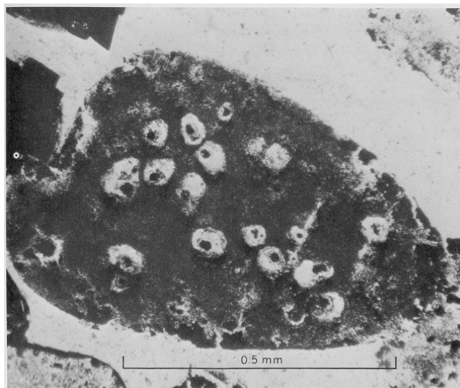
Figure 4.--Photomicrograph showing chert granule (dark gray) containing transparent structures, each having an opaque "nucleus." The darkest material is mostly hematite. Hematitic granular cherty iron-formation from Anvil Member, Ironwood Iron-formation; NW¼NW¼ sec. 13, T. 47 N., R. 46 W., near Ramsay, Mich.; plane-polarized light.
