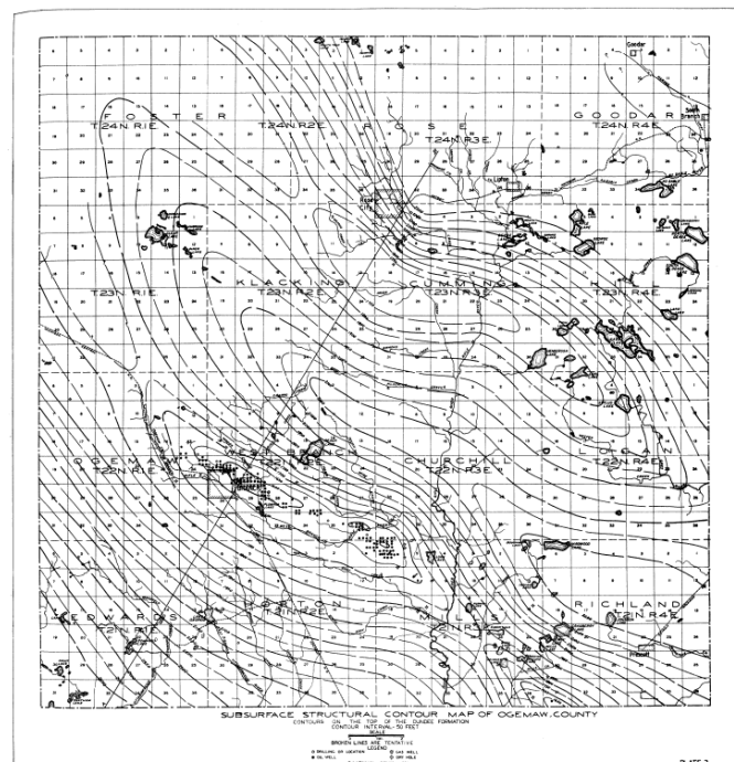
Plate 3. Subsurface structural contour map of Ogemaw County.
