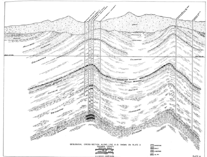
Plate 4. Geological cross-section along Line A-B shown on Plate 3.
