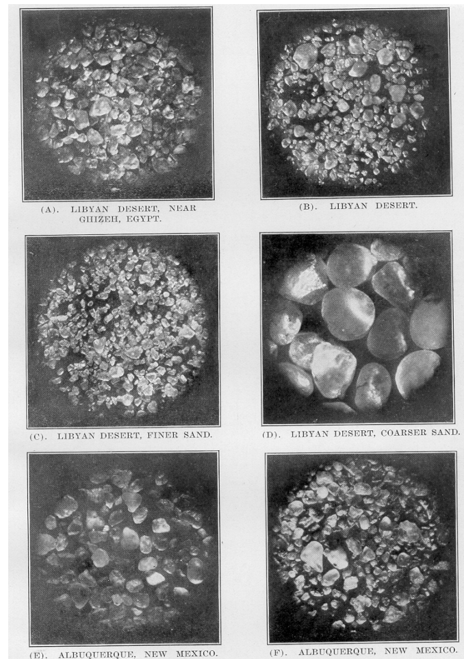
Plate VI. Desert sand grains, enlarged 14\frac{1}{2} times, showing the tendency of the wind to produce a sub-spherical type of granule. The finer, angular material present in the sand of modern deserts is believed to be due to accessions of new material or the continuance of residual action and consequent incompleteness of the aeolian agency.
