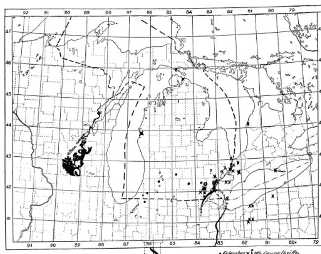
Figure 1. Map showing distribution of Sylvania Sandstone. (Base map by permission of Prof. M. S. W. Jefferson.)
