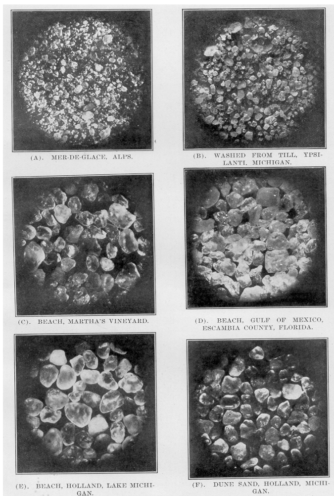
Plate V. Sand grains, enlarged 14\frac{1}{2} times, showing the passage from the sharp, fresh, glacially manufactured sand to the subangular and rounded varieties resulting from water and wind action.
