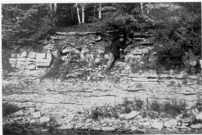
Thicker bed of limestone, just above center of picture, is top of Black River section. Shaly limestones of the Trenton appear just above the Black River. North of the bridge across the Escanaba River at Cornell.
