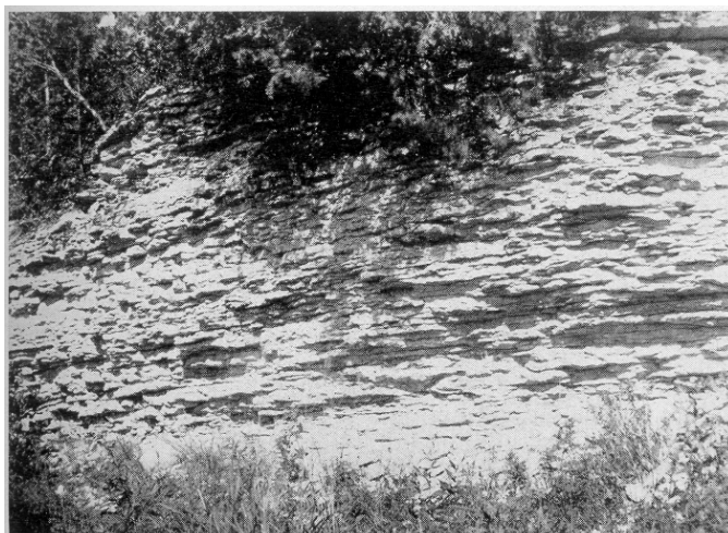
Unevenly bedded argillaceous limestone of the Maclurites zone north of the bridge at Cornell, Michigan. This rock forms the top of the Chandler Falls member of the Trenton at Chandler Falls.
