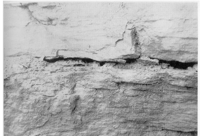
A layer of metabentonite, from two to three inches thick, may be seen just above the center of the picture. Trenton rock. Chandler Falls member at Chandler Falls.
