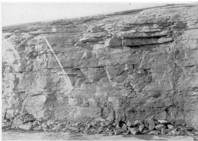
Trenton rock, Groos Quarry member, at the type locality in the abandoned Bichler quarry at Groos, Michigan. Thirty feet of rock are shown here.
