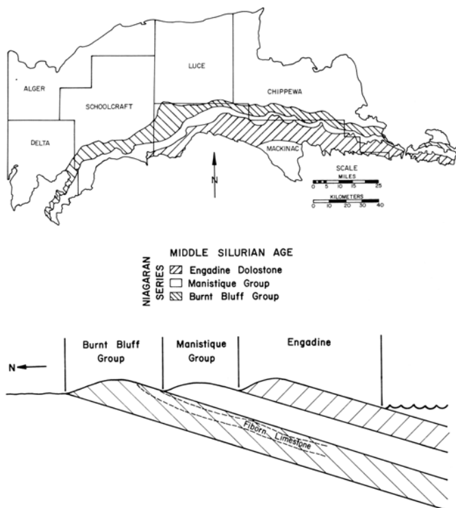
Figure 2. Geologic plan map with a generalized cross-sectional view.
