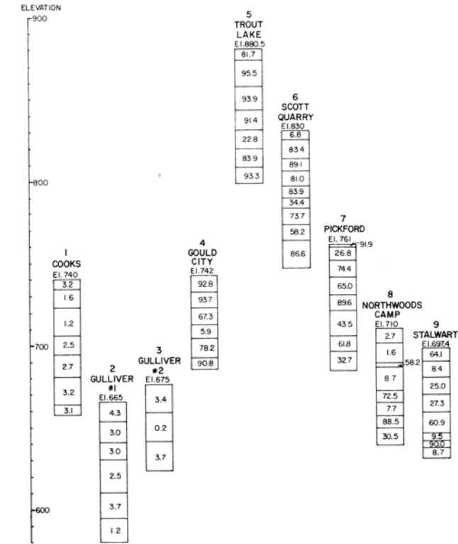
Figure 7. Strip logs showing elevation and calcite content for each sample interval.
