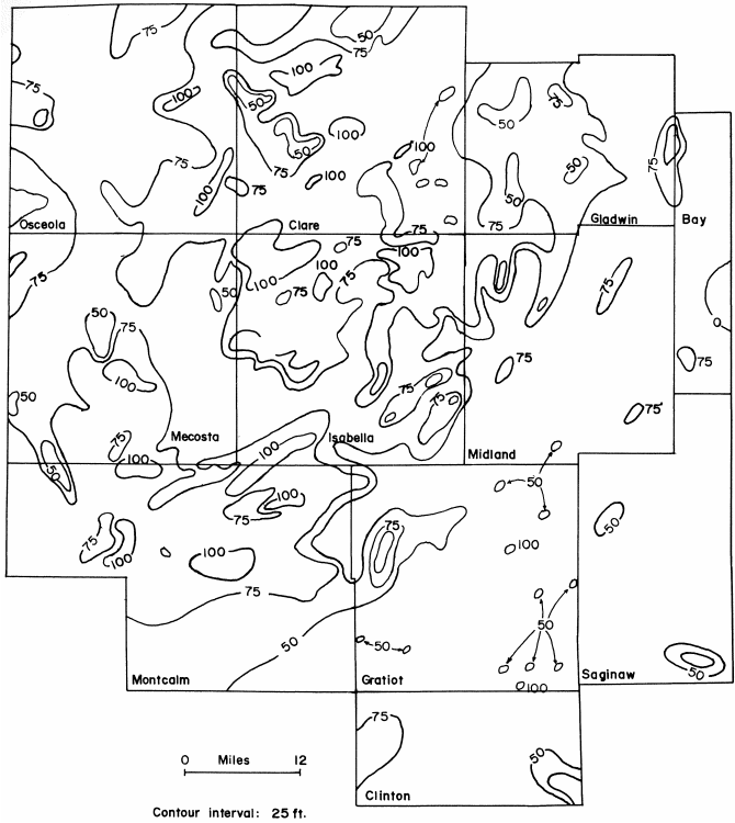
Figure 9. Isopach map of the Parma Formation.
