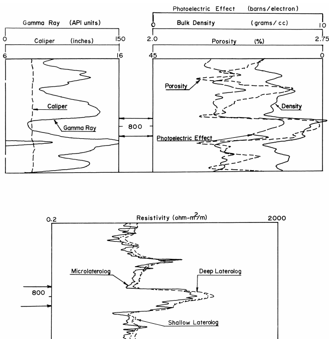
Figure 13. Geophysical logs from the well from which the type section of the Six Lakes Limestone member is taken.
