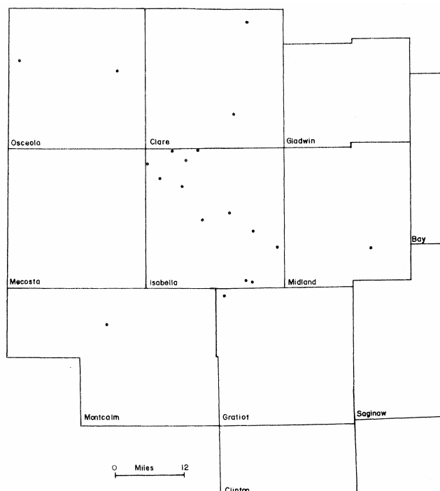
Figure 2. Location of geological test wells from which drill cuttings were examined.
