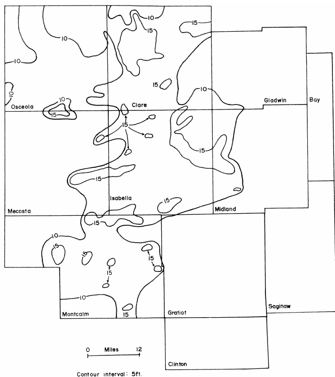
Figure 5. Isopach map of the middle unit of the Bayport Formation.
