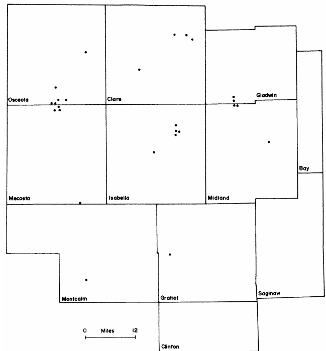
Figure 22. Location of wells in which coal is indicated by geophysical logs.
