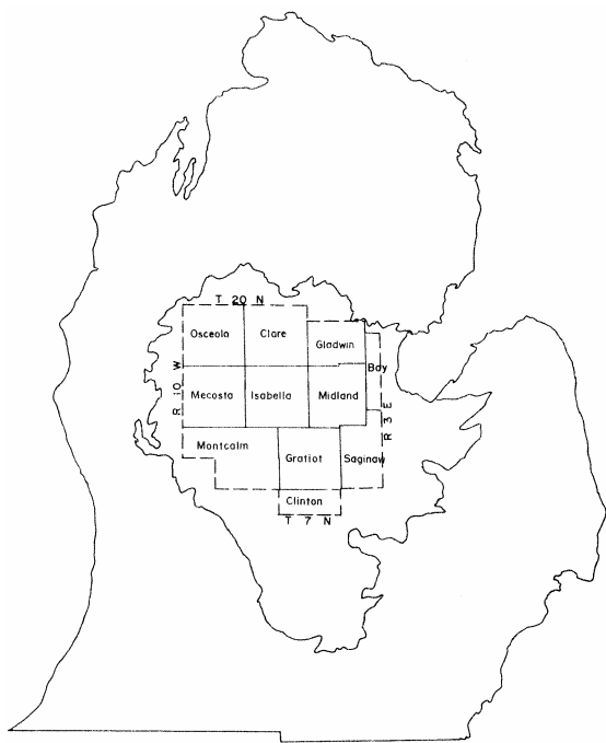
Figure 1. Study area and limit of Pennsylvanian rocks in Michigan.
