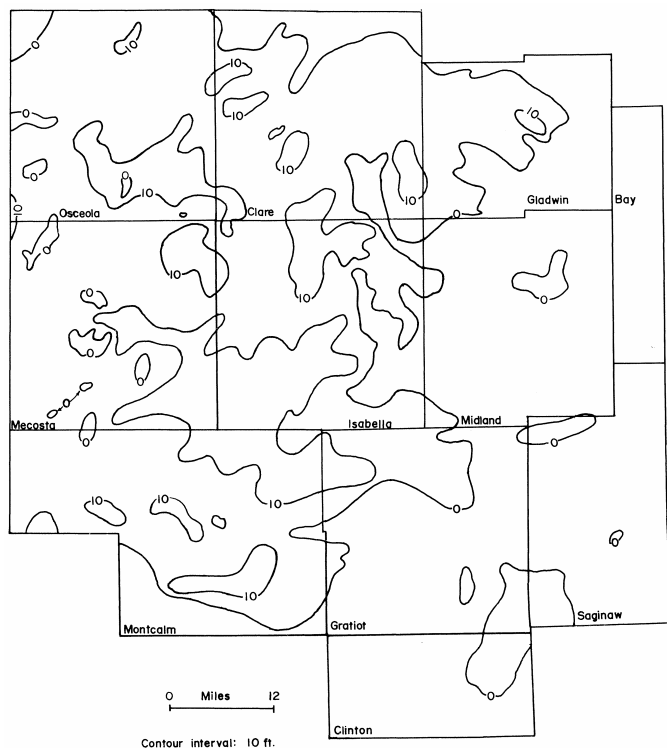
Figure 14. Isopach map of the Six Lakes Limestone Member.
