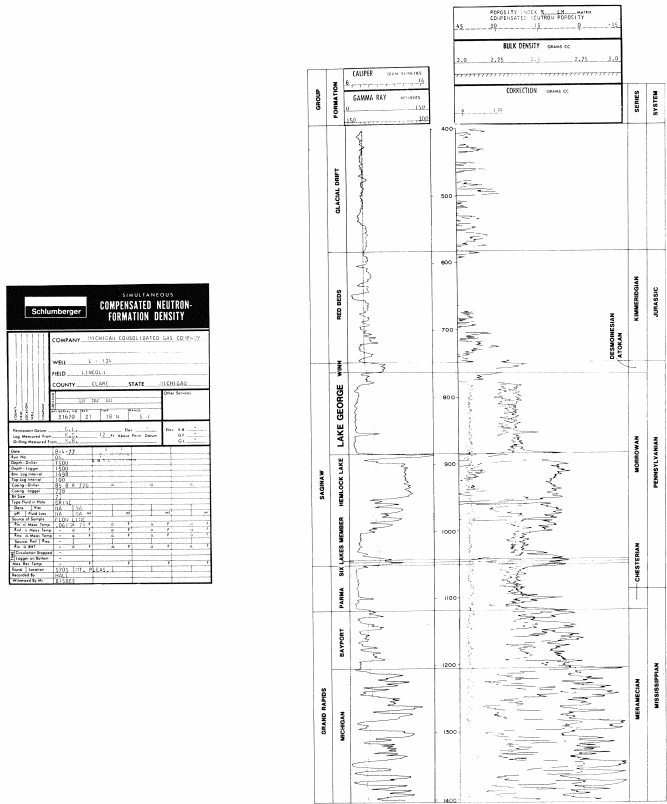
Figure 17. Geophysical logs from the well from which the type section of the Lake George Formation is taken.
