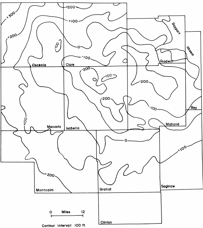
Figure 10. Structural contours on the top of the Bayport Formation.
