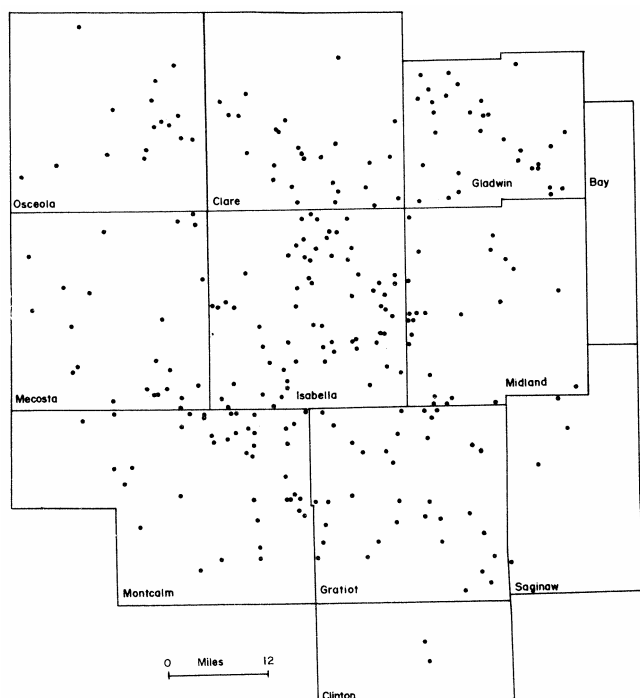
Figure 3. Location of wells from which only driller's logs are available.
