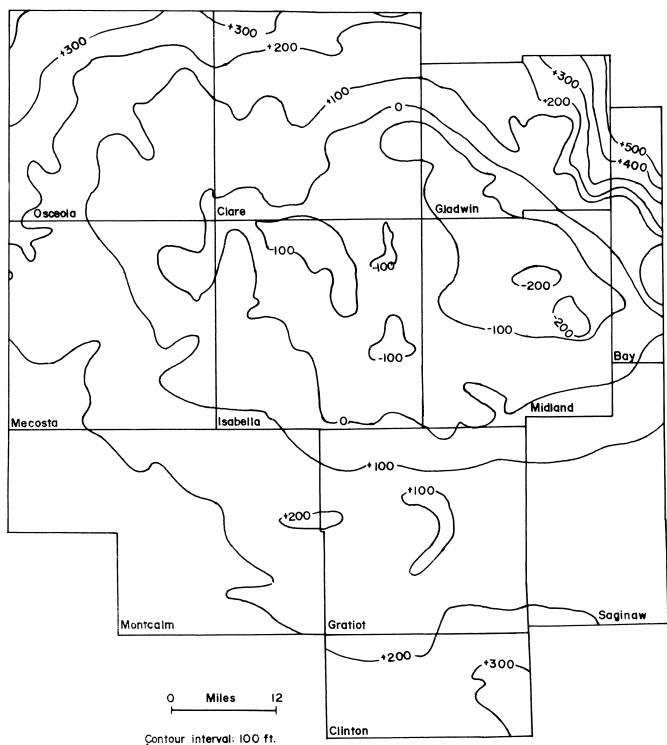
Figure 16. Structural contours on the base of the Hemlock Lake Formation.
