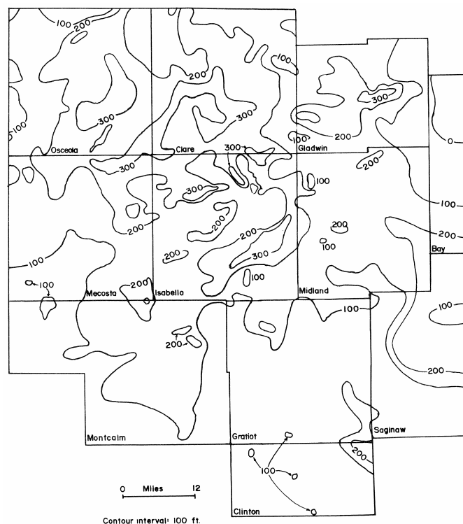
Figure 15. Isopach map of the Hemlock Lake Formation.
