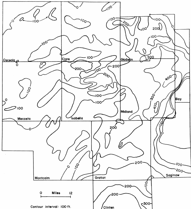
Figure 18. Isopach map of the Lake George Formation.
