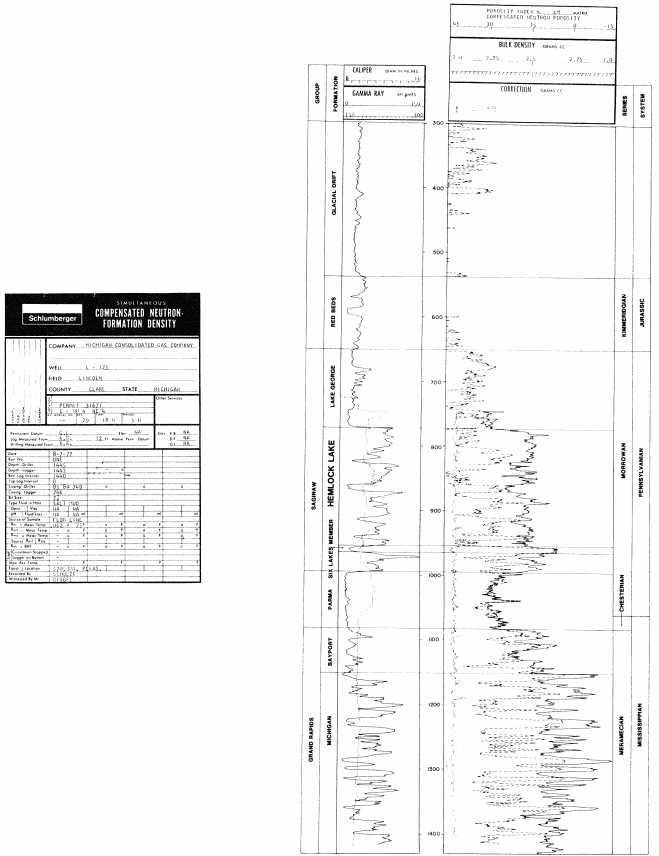
Figure 11. Geophysical logs from the well from which the type section of the Hemlock Lake Formation is taken.
