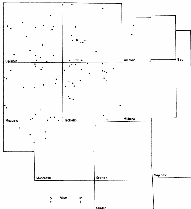
Figure 7. Location of wells in which the top of the Michigan Formation is marked by an anhydrite bed.
