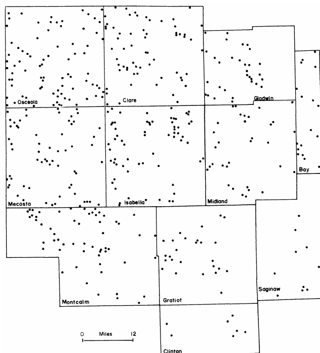
Figure 4. Location of wells from which geophysical logs are available.
