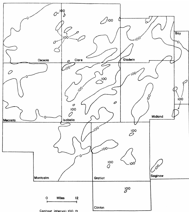
Figure 20. Isopach map of the Winn Formation.
