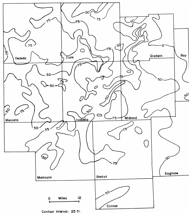
Figure 6. Isopach map of the Bayport Formation.
