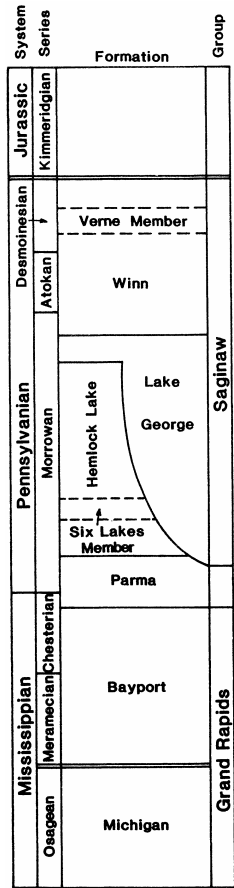
Figure 23. Generalized relationships between Carboniferous rock-stratigraphic and time-stratigraphic units in Michigan.
