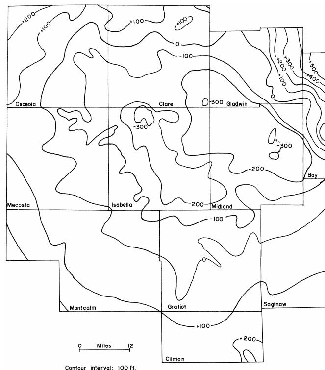
Figure 8. Structural contours on the top of the Michigan Formation.
