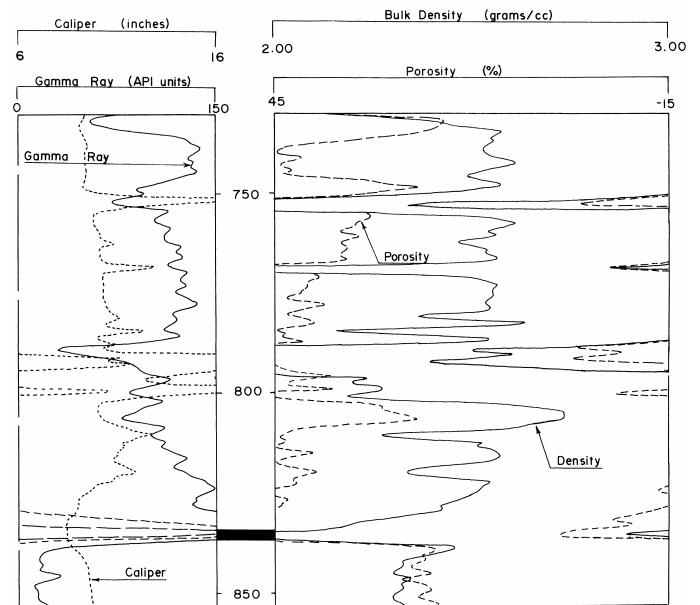
Figure 12. Geophysical logs showing a thin coal at the base of the Hemlock Lake Formation.
