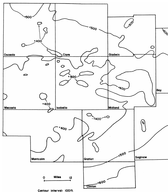
Figure 21. Structural contours on the top of the Pennsylvanian System.
