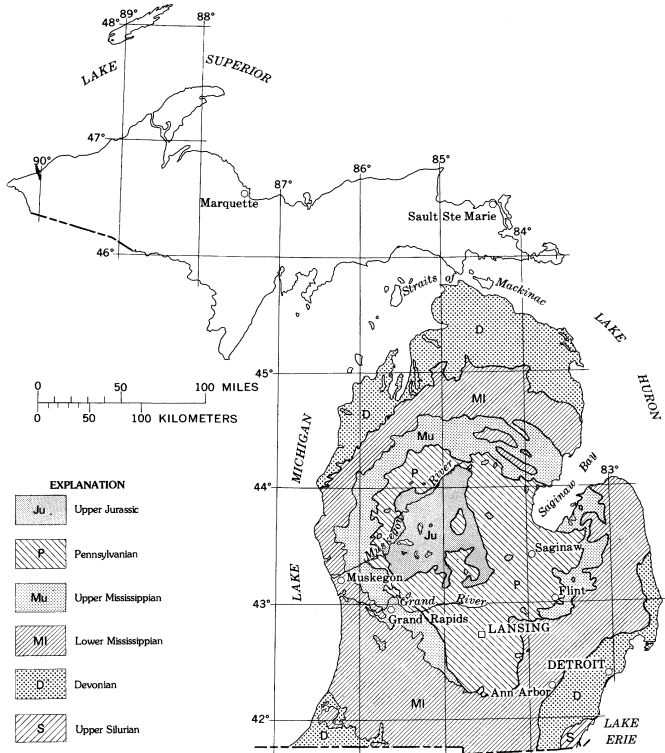
FIGURE 1.—Distribution of Mississippian, Pennsylvanian, and remnant Jurassic bedrock in the Southern Peninsula of Michigan. Jurassic rocks overlie a part of the Pennsylvanian section and are limited to the basin interior. Outermost bedrock areas of the Southern Peninsula are Devonian except for a small area of Upper Silurian strata near the western end of Lake Erie. Distribution of bedrock units adapted from Kelley (1968).
