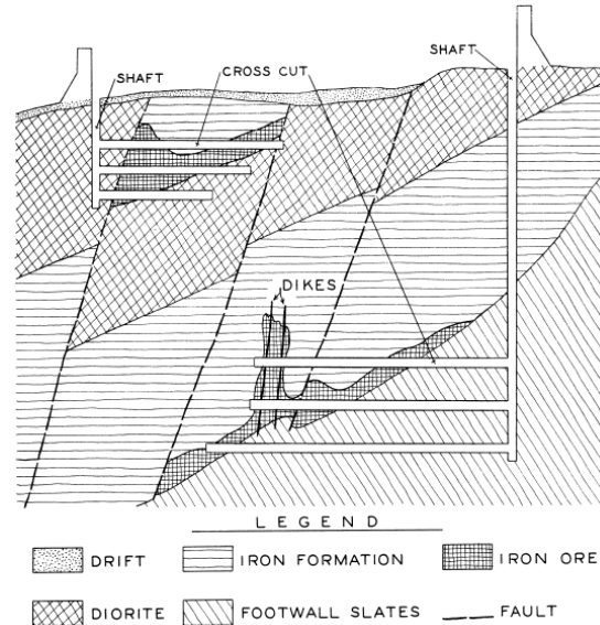
Figure 7. Generalized geologic cross section of the Marquette Iron Range.
