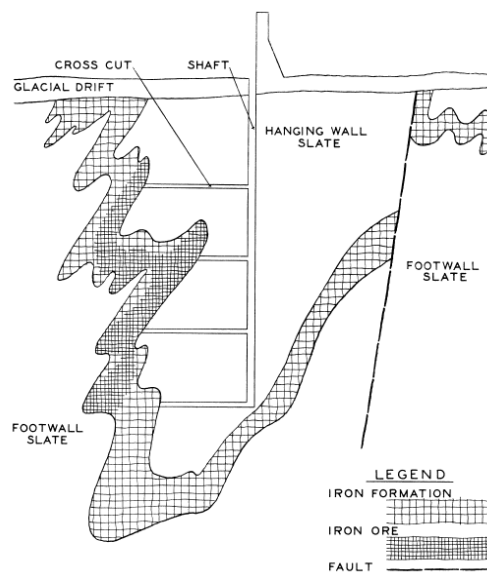
Figure 14. Generalized geologic cross section, Iron River – Crystal Falls Iron Range
