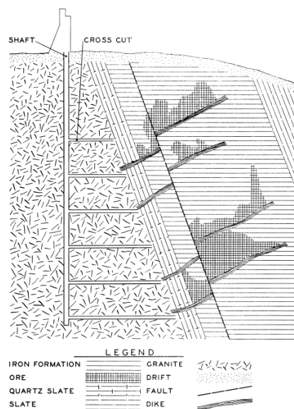
Figure 18. Generalized geologic cross-section, Gogebic Iron Range
