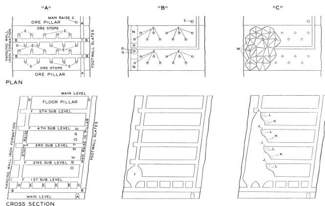
Figure 15. Mining by sub-level stoping, Iron River – Crystal Falls Iron Range
