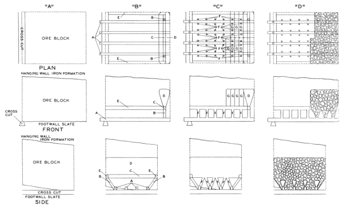
Figure 8. Mining by block caving, Marquette Iron Range.
