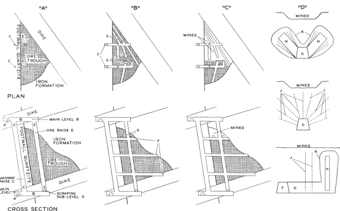
Figure 19. Mining by sub-level caving, Gogebic Iron Range
