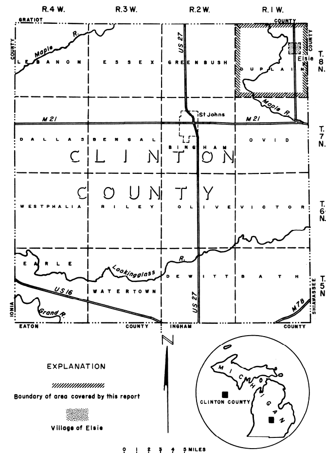
Figure 1. Index map showing location of the Elsie area, Michigan
