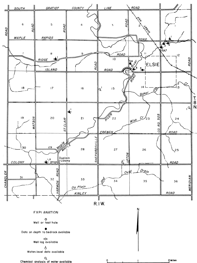
Figure 3. Map of Duplain Township showing location of wells outside the village of Elsie
