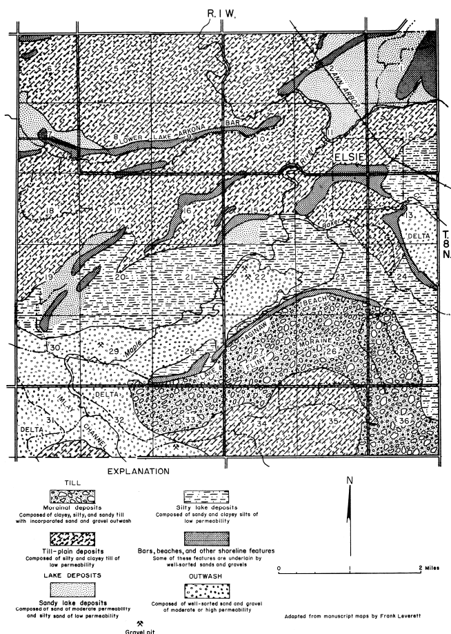
Figure 5. Surficial geology of the Elsie area
