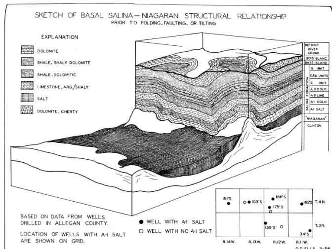
Figure 10. Sketch of basal Salina-Niagaran structural relationship.
