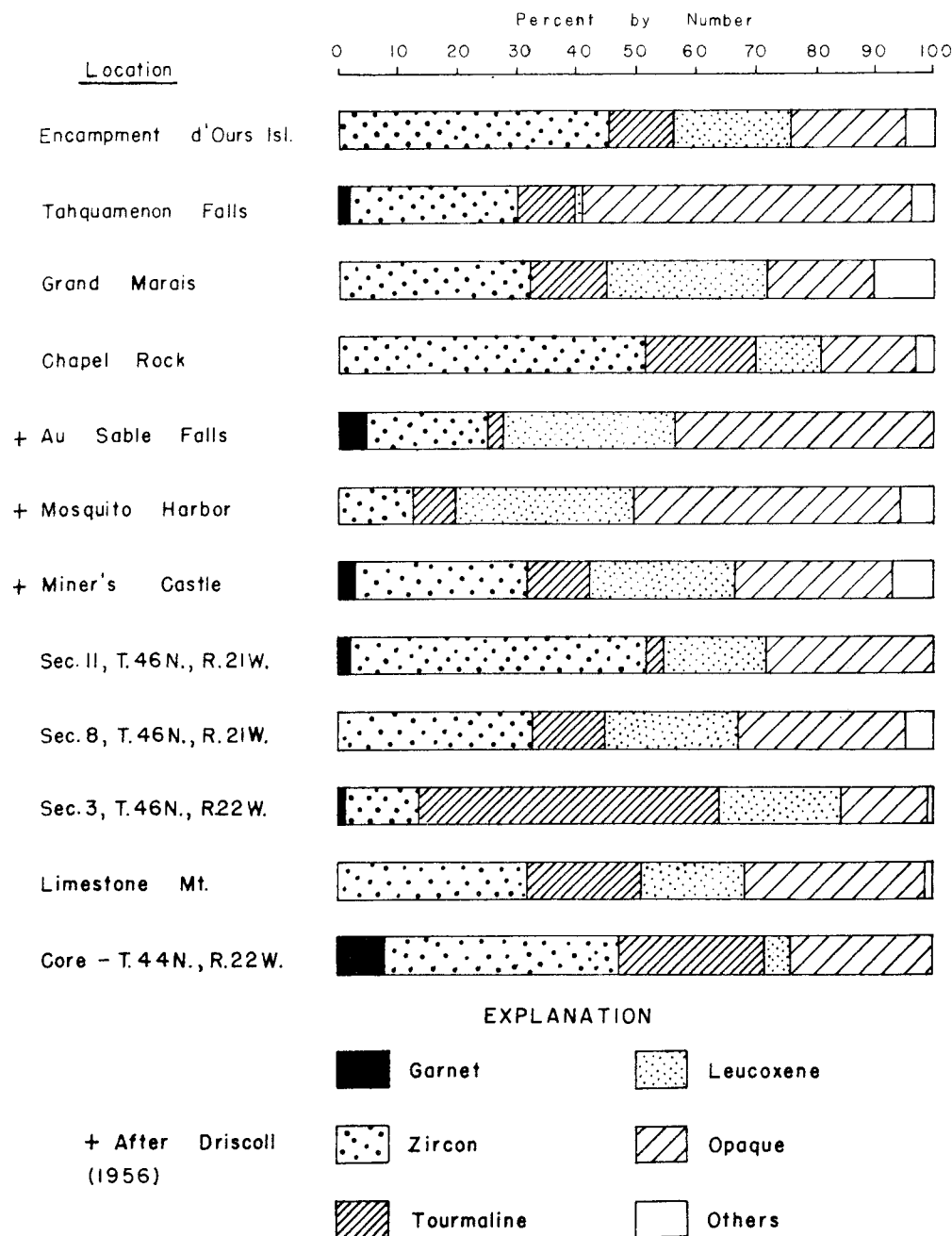
Figure 43. Heavy minerals of the Chapel Rock member
