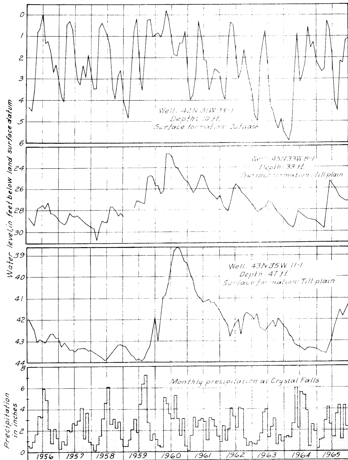
Figure 3. Fluctuations of ground-water levels.
