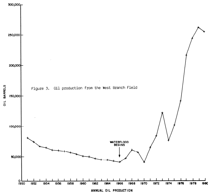
[Figure 3. Oil Production from the West Branch Field]
