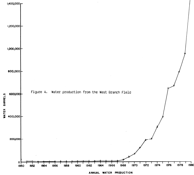
[Figure 4. Water production from the West Branch Field]
