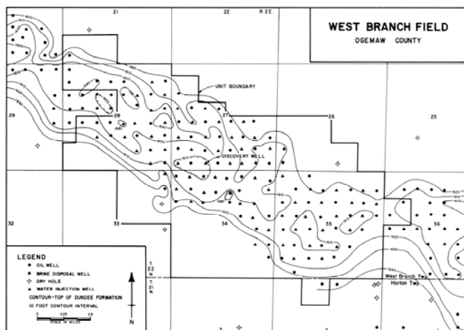
Figure 2. Structure of the West Branch Field contoured on the top of the Dundee Formation
