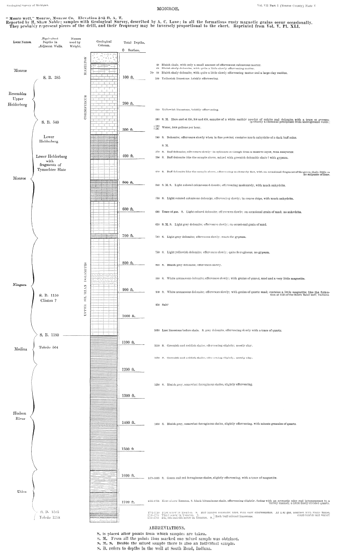
Plate V. Section of the Monroe well (from Vol. V.)
