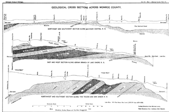
Plate VI. Cross sections along line of railroads.
