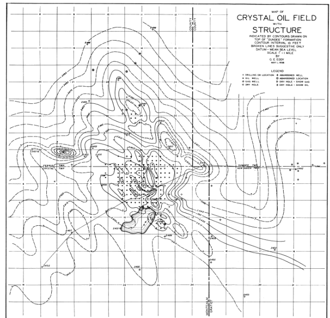
Figure 1. Map of Crystal Oil Field with structure indicated by contours drawn on the top of "Dundee" formation. By G. E. Eddy, May 1, 1936.
