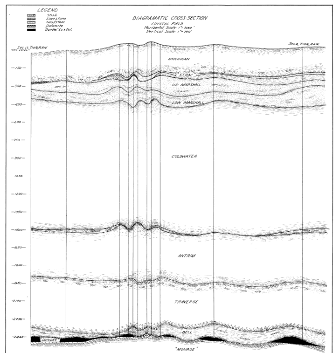
Figure 2. Diagrammatic cross-section, Crystal Field.
