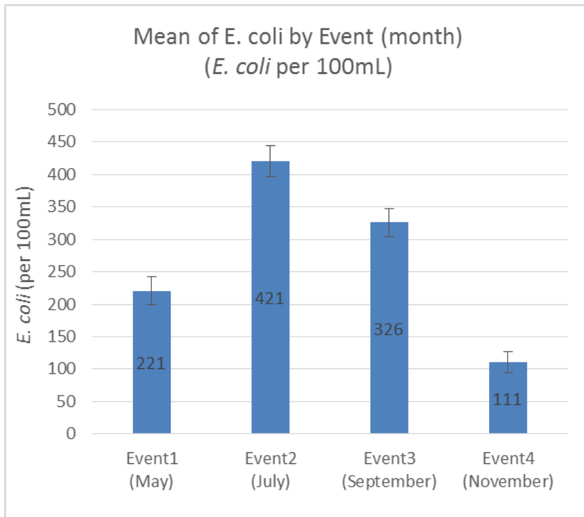
Figure 42. Mean of WCMP E. coli data pooled by event across all years (2009, 2011, 2012, and 2013).
