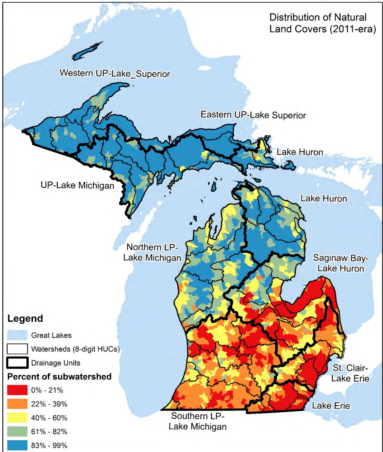
Figure 4. Natural land cover distribution (2011-era) as a percent of each subwatershed (NOAA, 2011). All forested, scrub, grassland, and wetland land cover types are included.
