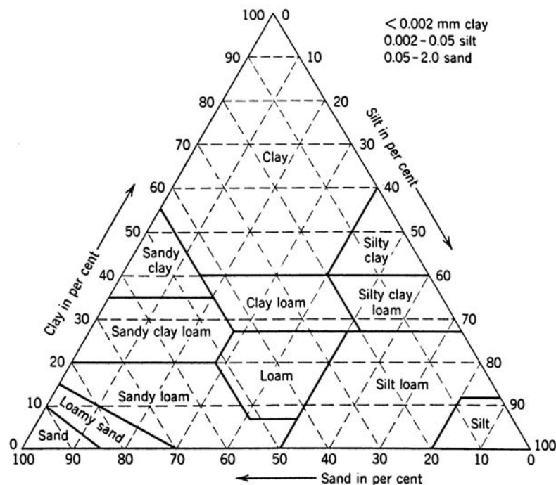
Figure 1-5 Textural Triangle
