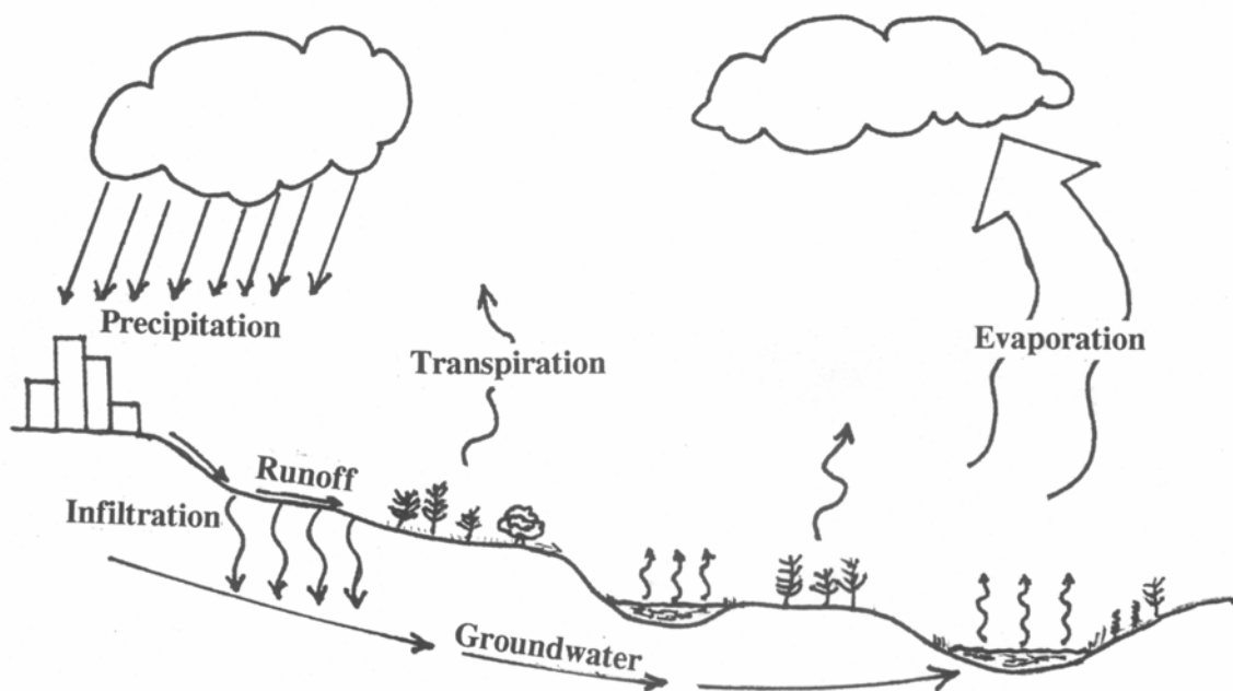
Figure 1.1 Hydrologic Cycle
