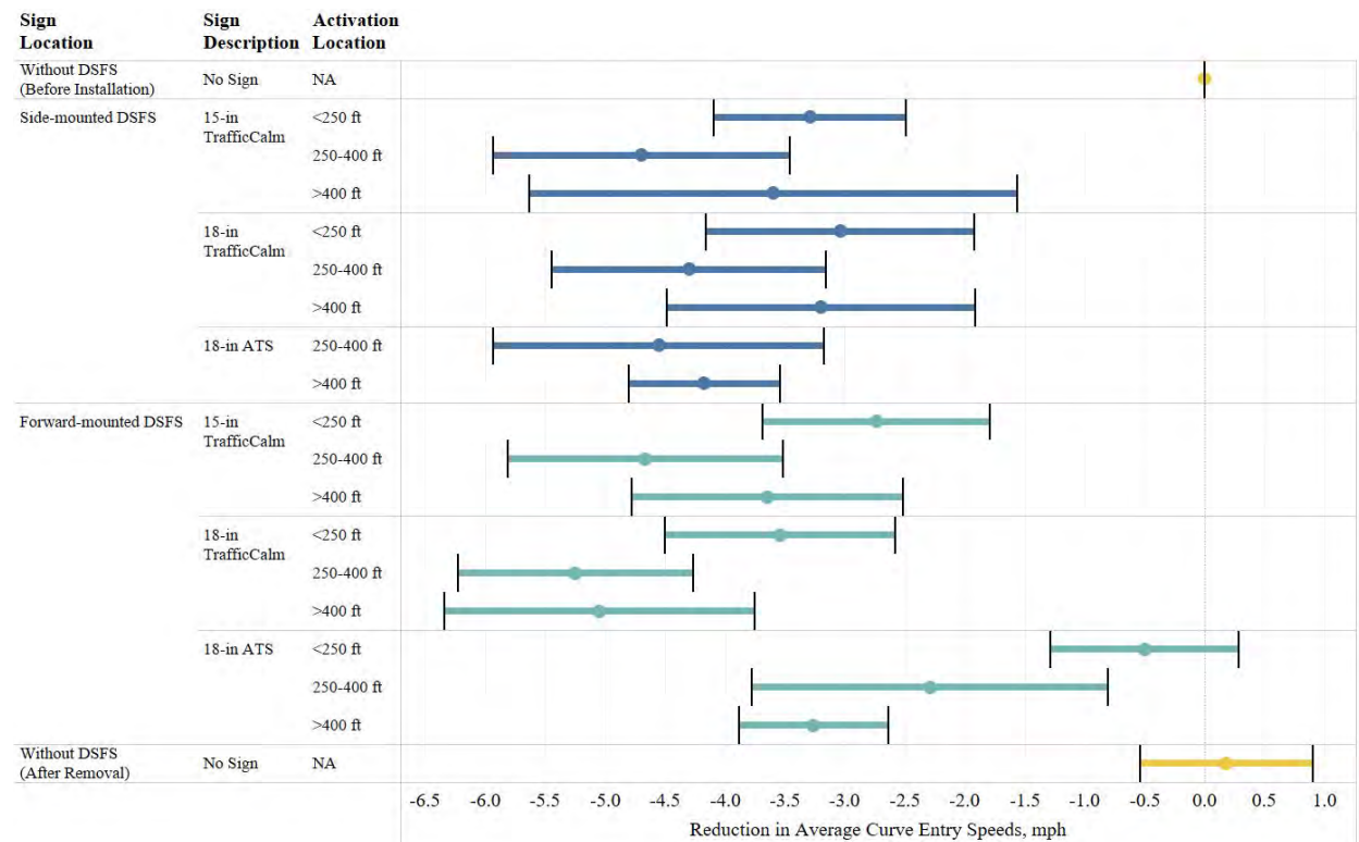
Figure 23. Linear regression parameter estimates for the reduction in curve entry speed (with 95% confidence intervals)
